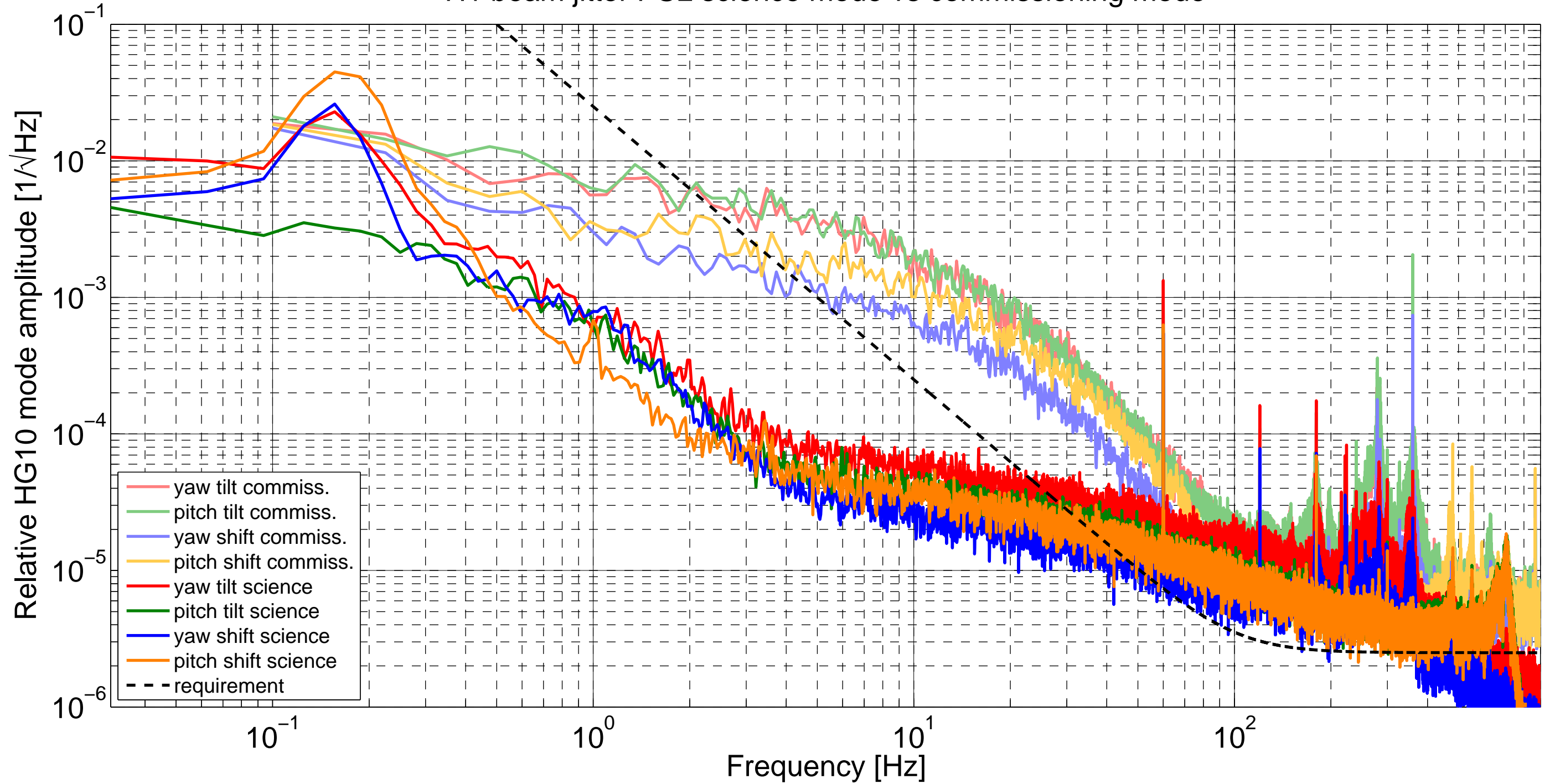
H1 beam jitter PSL science mode vs commissioning mode
