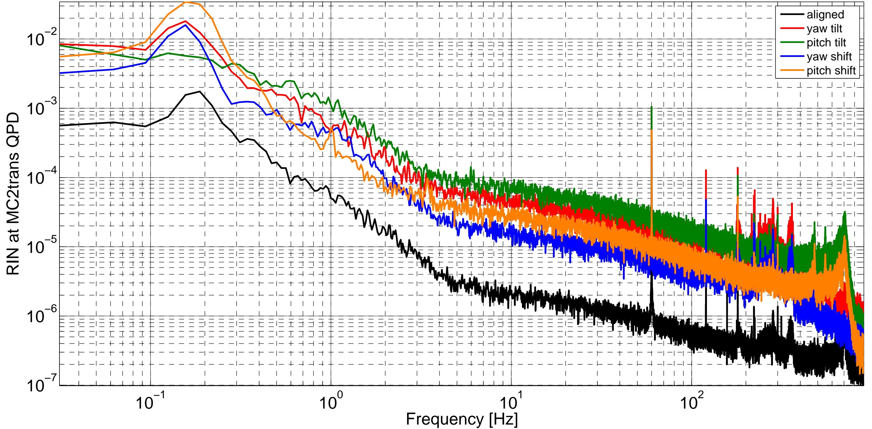
RIN spectra for aligned and misaligned IMC
