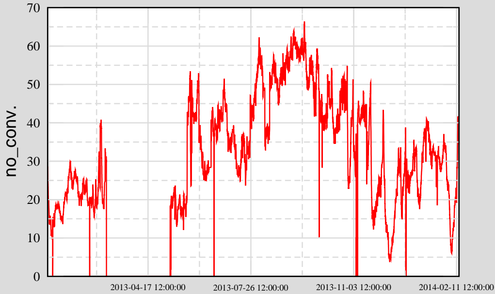
Ch 3: H1:PSL-ENV_CHILLERM_RH
