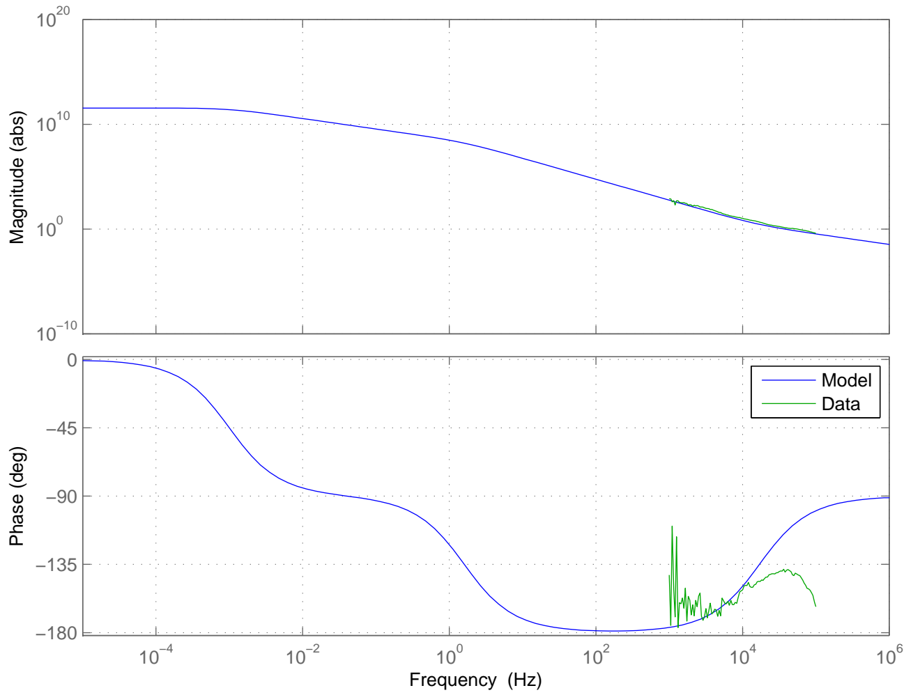
COMM PLL to VCO Open Loop TF
