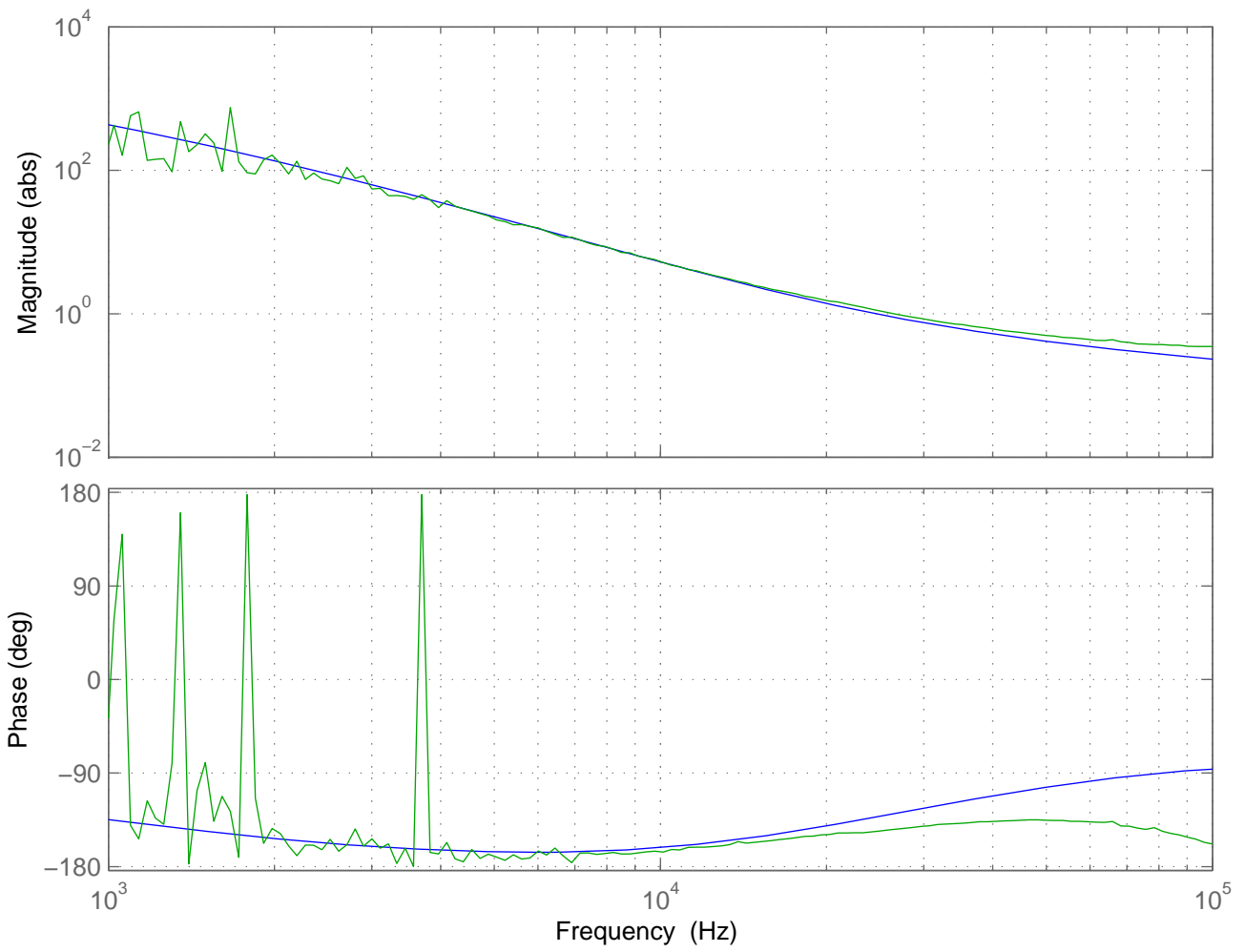
IMC Common Path OLTF
