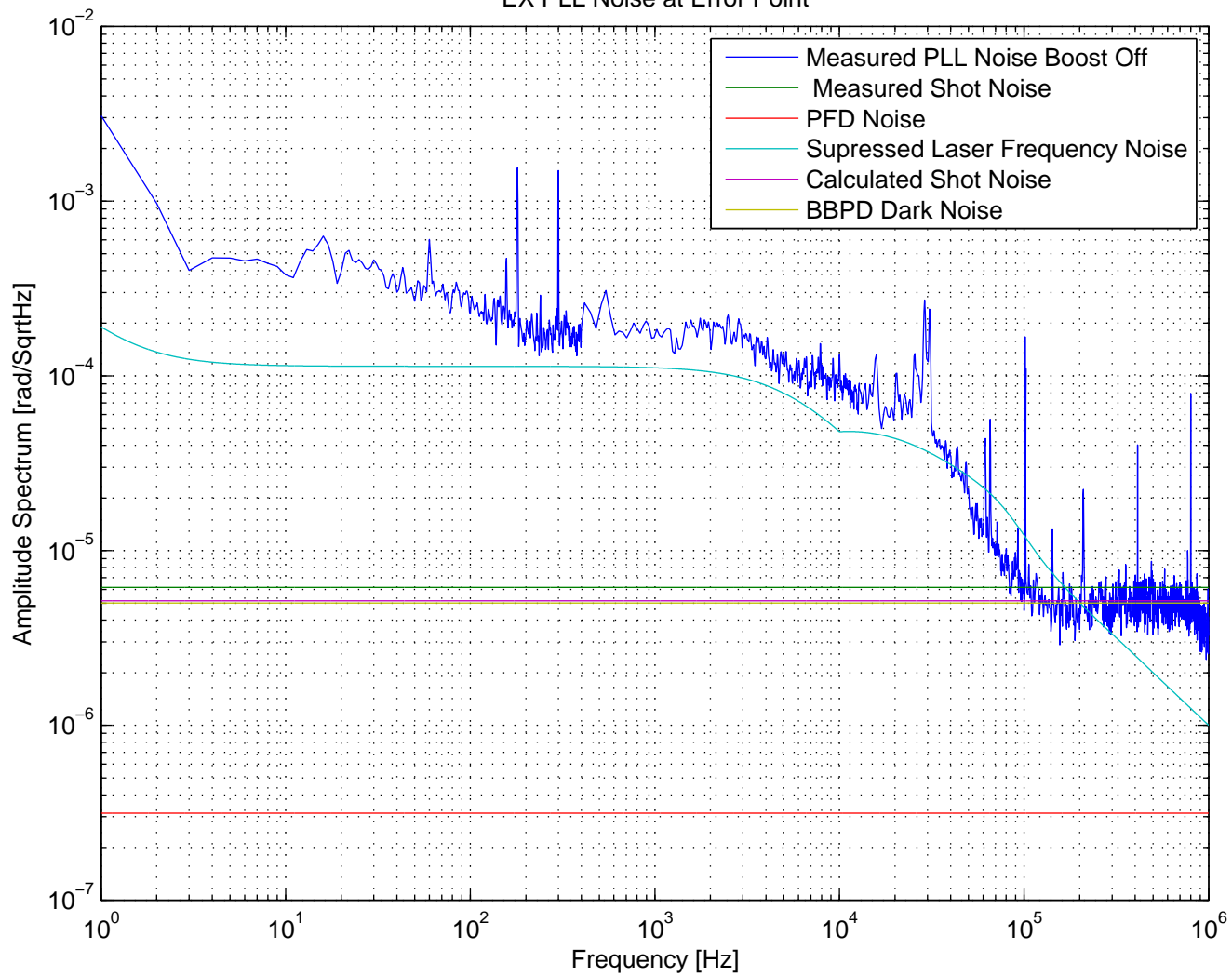
EX PLL Noise at Error Point
