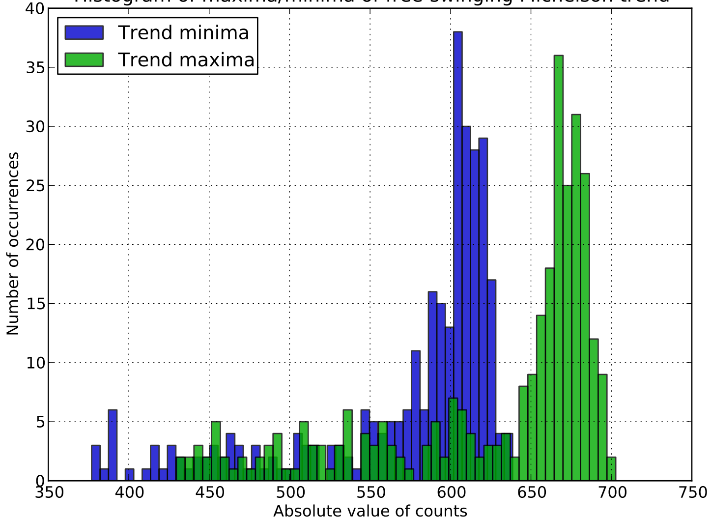
Histogram of maxima/minima of free-swinging Michelson trend
