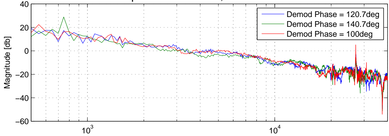
Mod Freq = 24.407363Mhz, Diff Demod Phase
