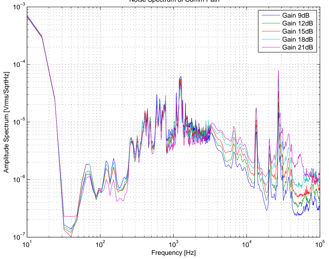
Noise Spectrum of Comm Path
