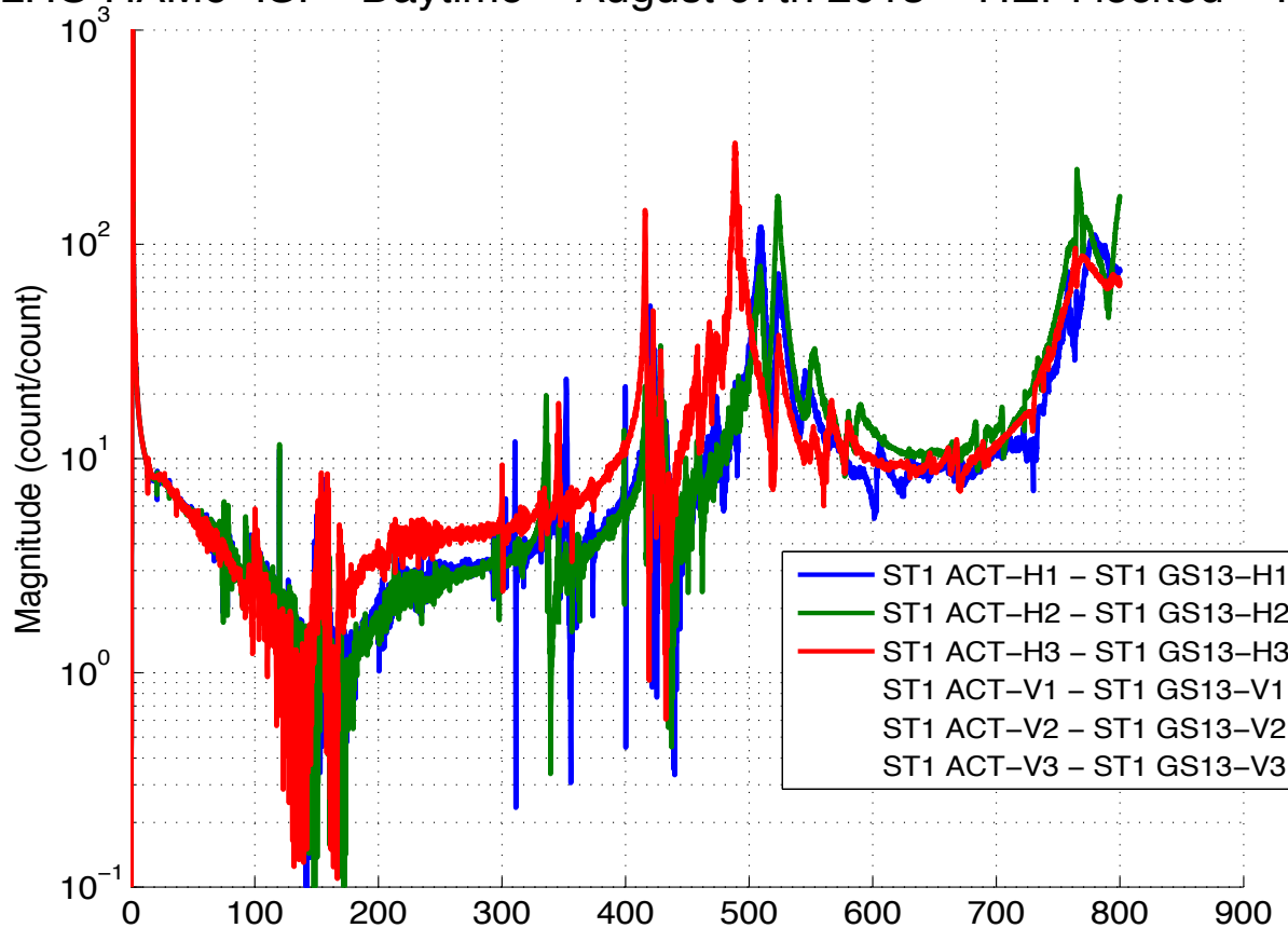
LHO HAM6-ISI – Daytime – August 07th 2013 – HEPI locked – In Air
