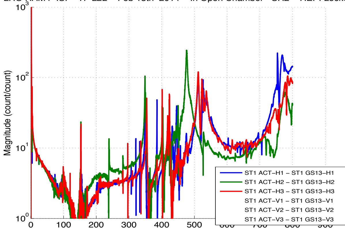
LHO HAM4-ISI – TF L2L – Feb 13th 2014 – In Open Chamber –SR2 – HEPI Locked
