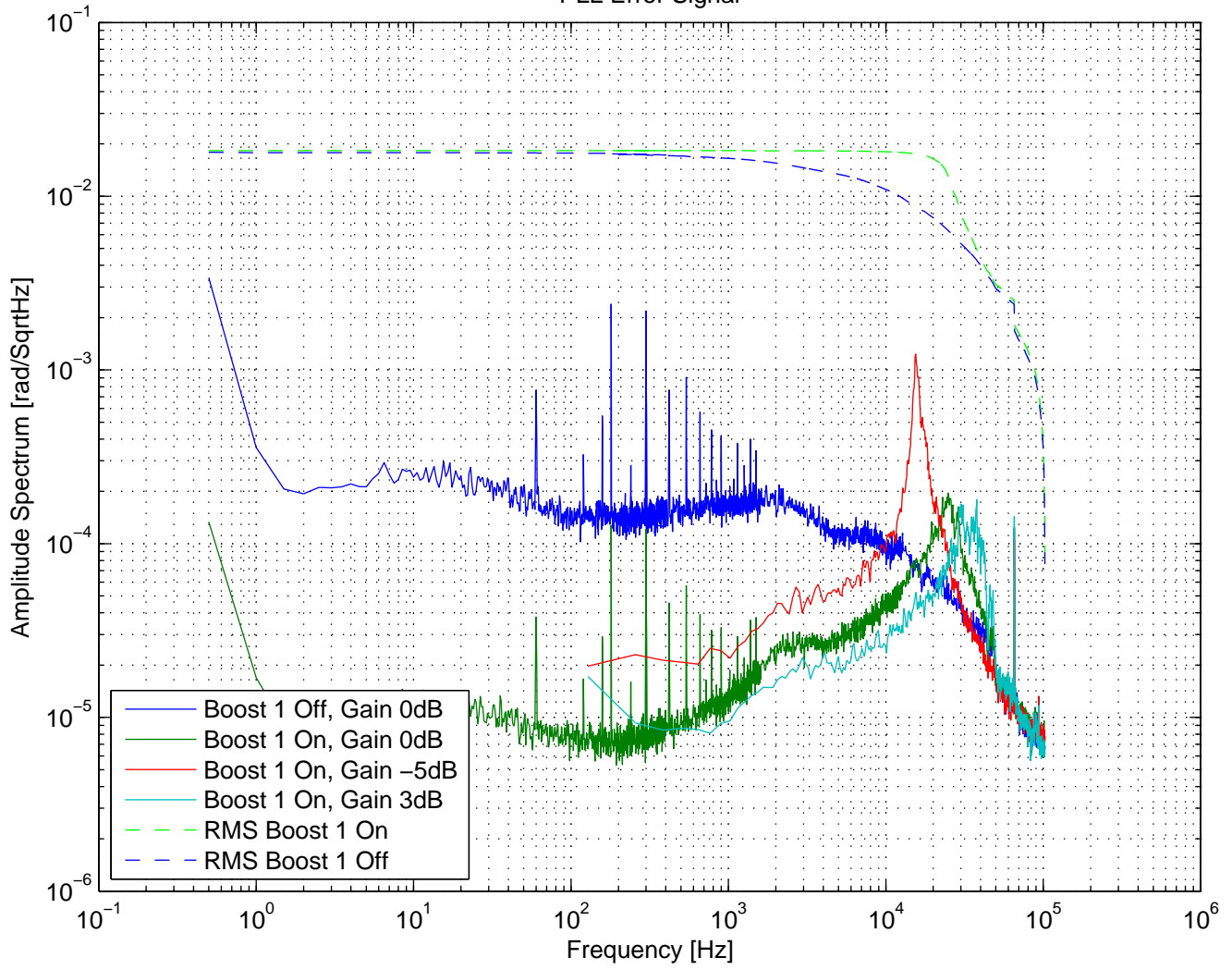
PLL Error Signal
