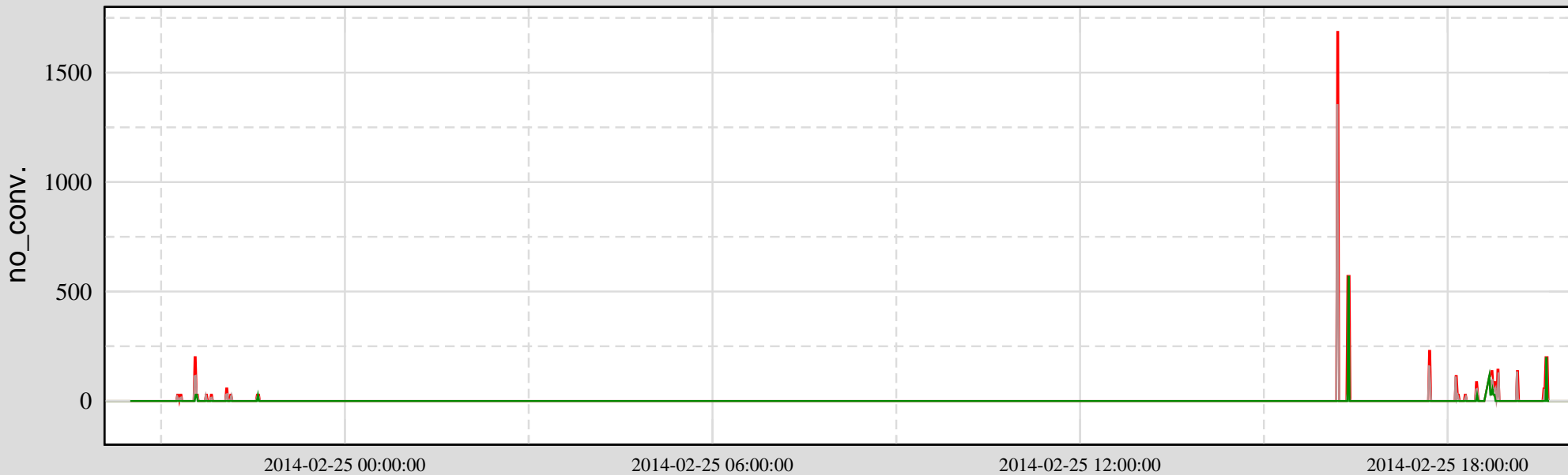
Ch 2: H0:PEM-EY_DUST_VEA1_500NM_PCF
