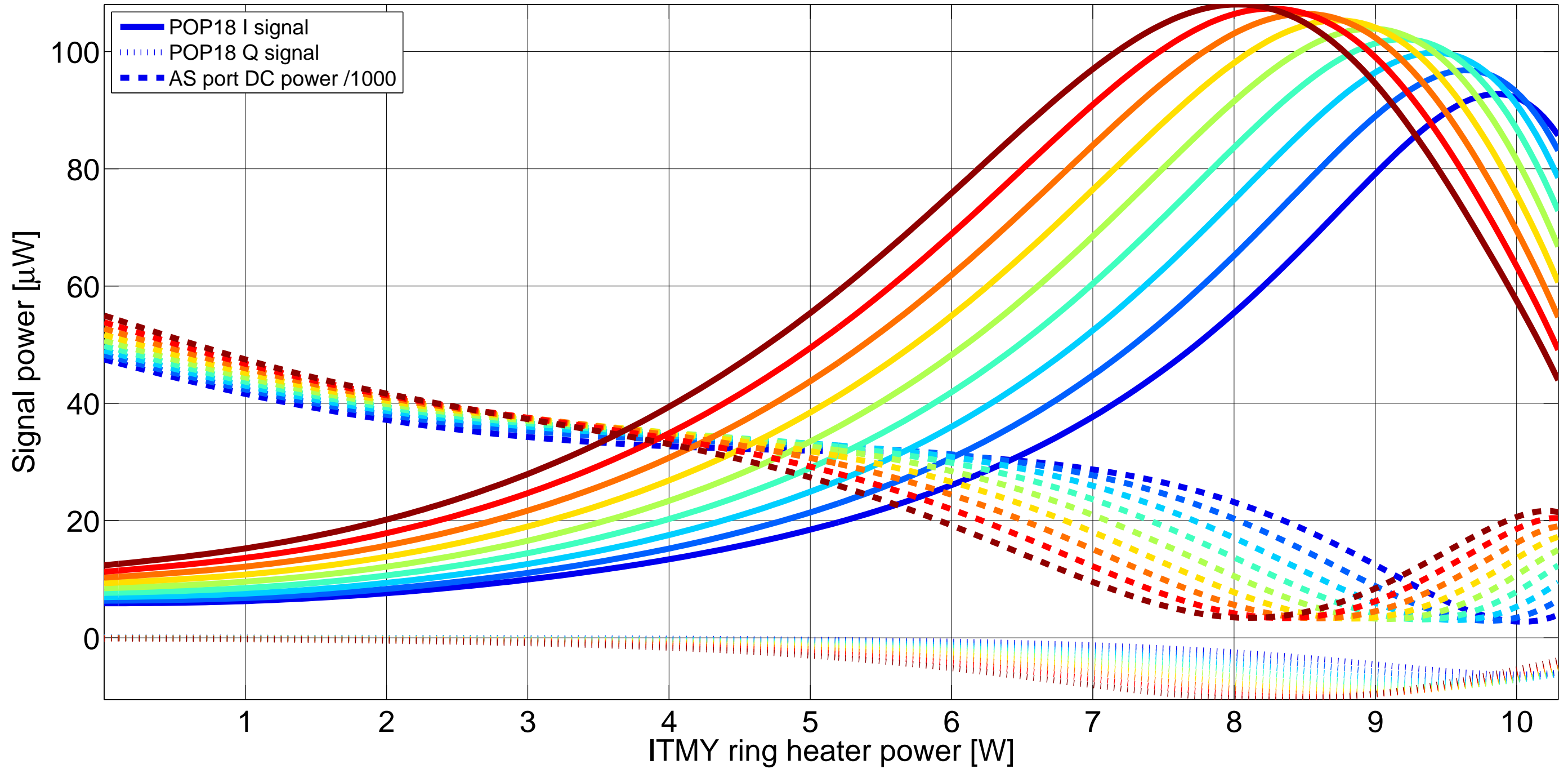
H1 SB PRMI signals with ITMY RH, various ITMX nonTL values (blue = -15\mu\text{D} to brown = +15\mu\text{D} )
