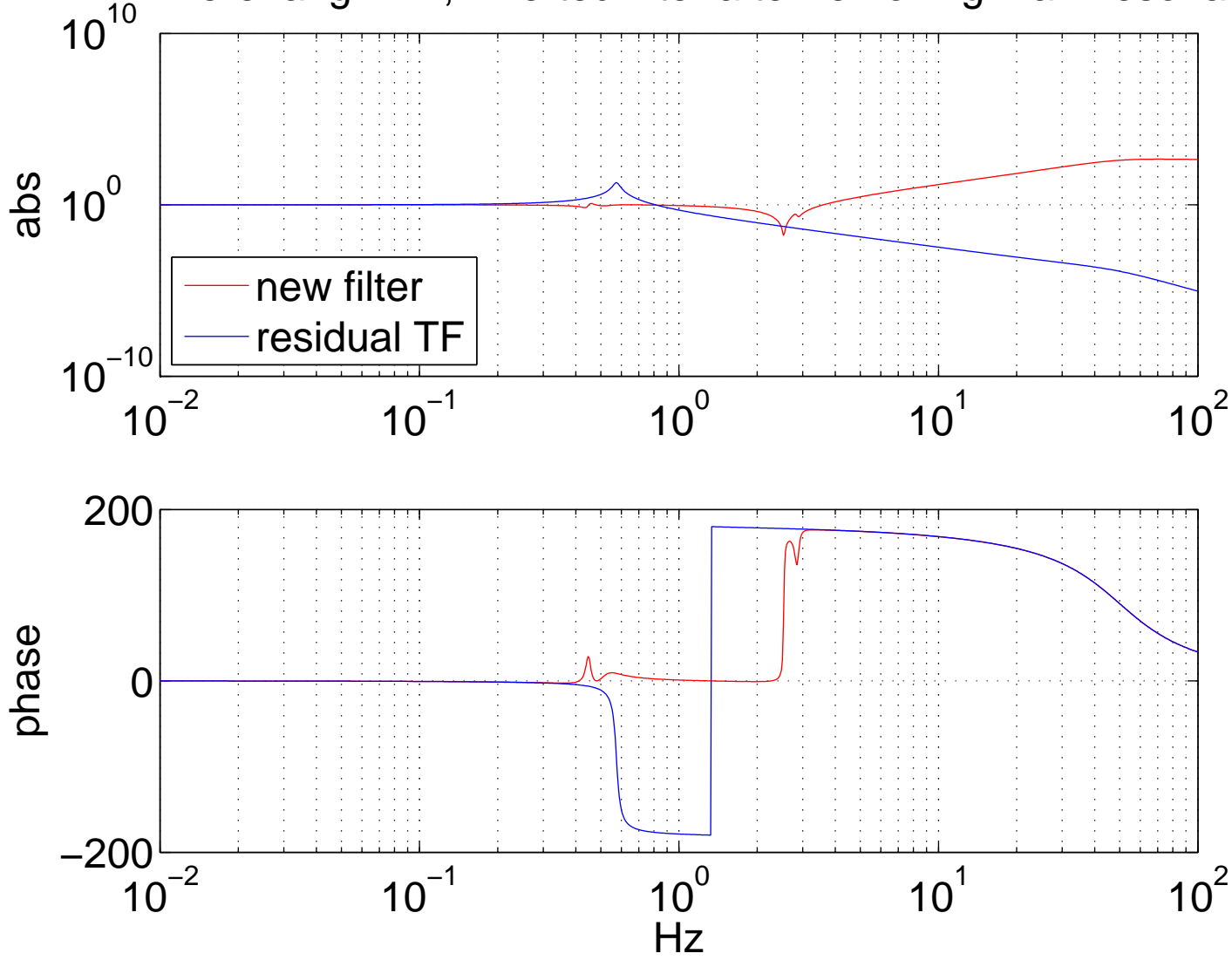
ITM wirerehang P2P, inverted filter after removing main resonance.
