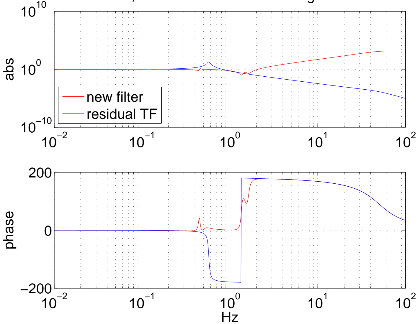
ETM fiber P2P, inverted filter after removing main resonance.
