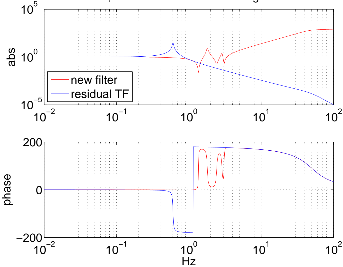
ETM fiber Y2Y, inverted filter after removing main resonance.
