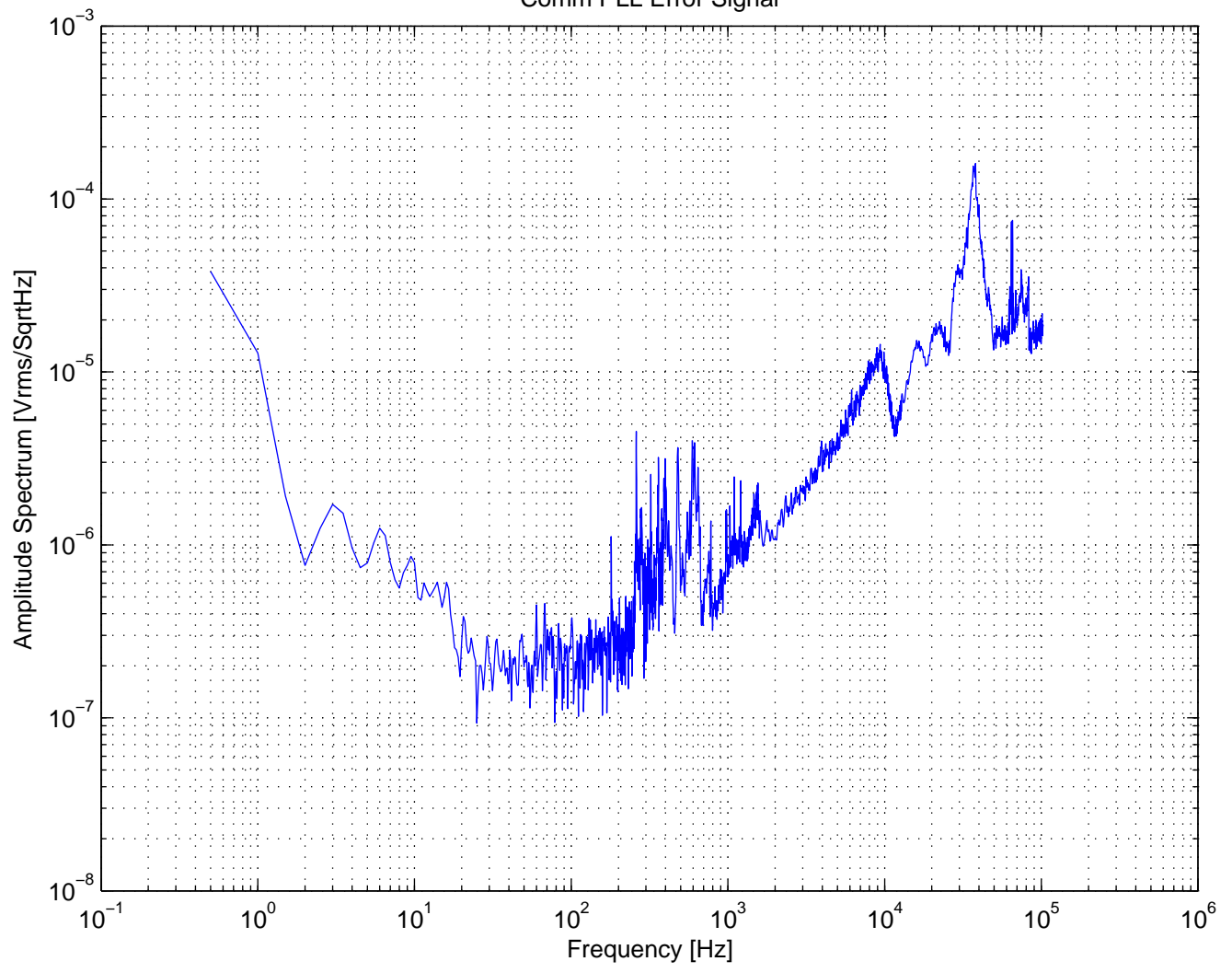
Comm PLL Error Signal
