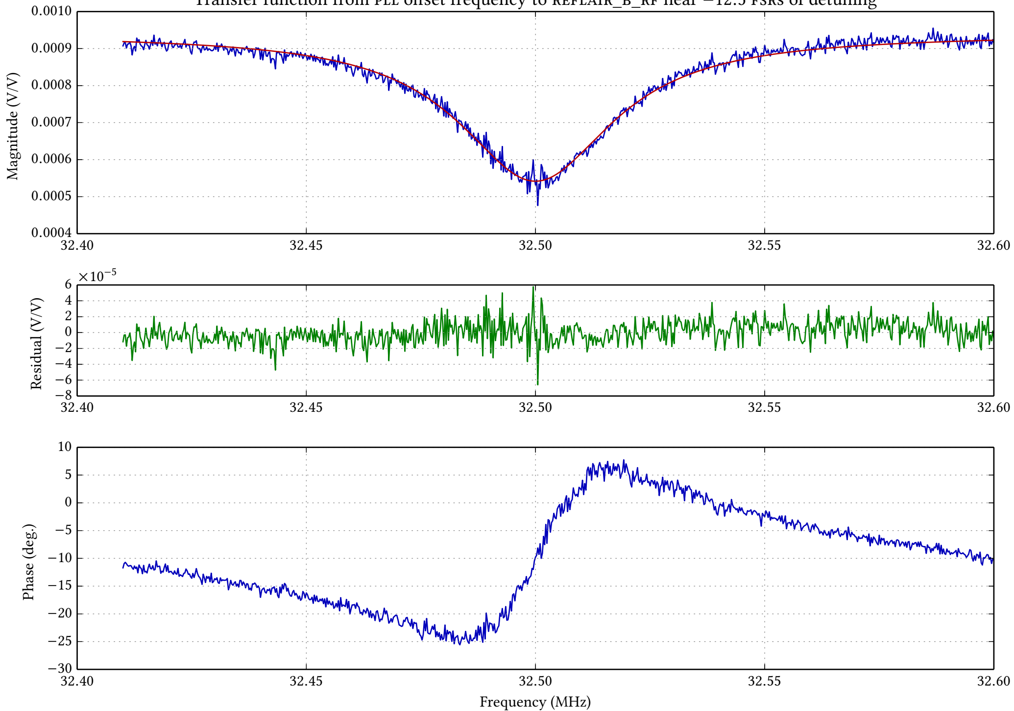
Transfer function from PLL offset frequency to REFLAIR_B_RF near -12.5 FSRs of detuning
