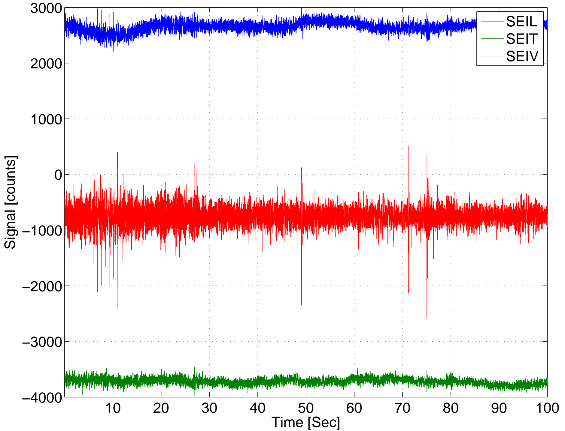
994714072 LHO H0 PEM LVEA Seismometer Time Series
