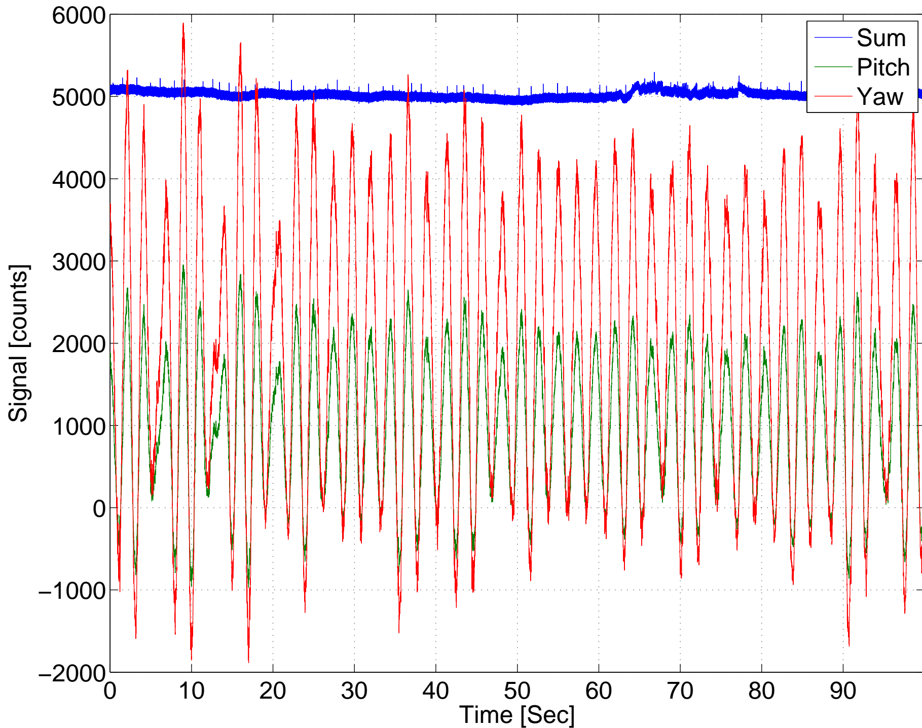
994714072 LHO H2 ITMY L3 Optical Lever Time Series
