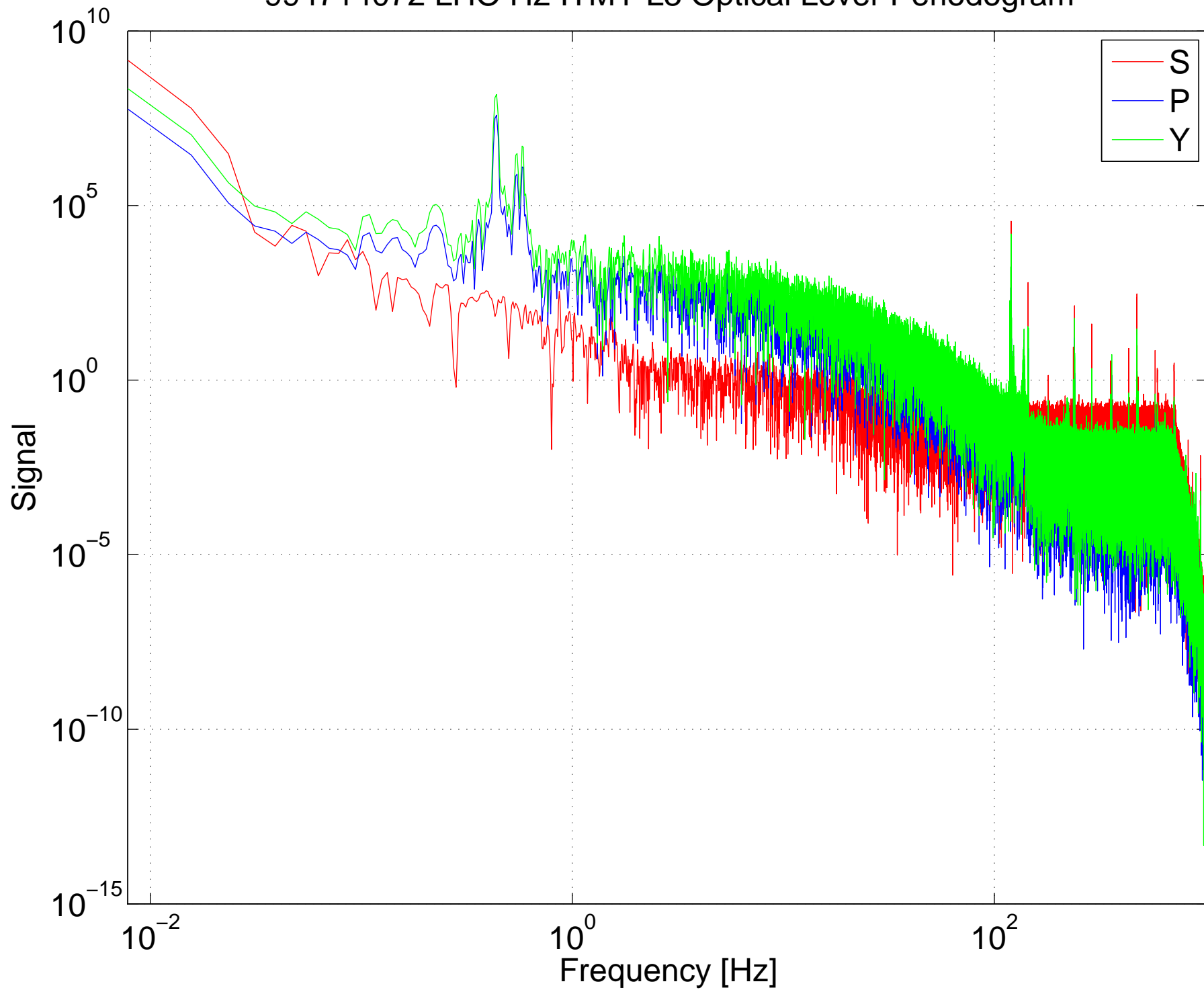
994714072 LHO H2 ITMY L3 Optical Lever Periodogram
