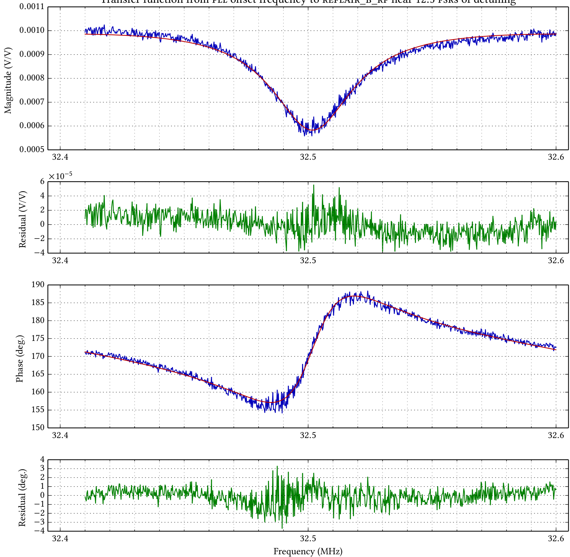
Transfer function from PLL offset frequency to REFLAIR_B_RF near 12.5 FSRs of detuning
