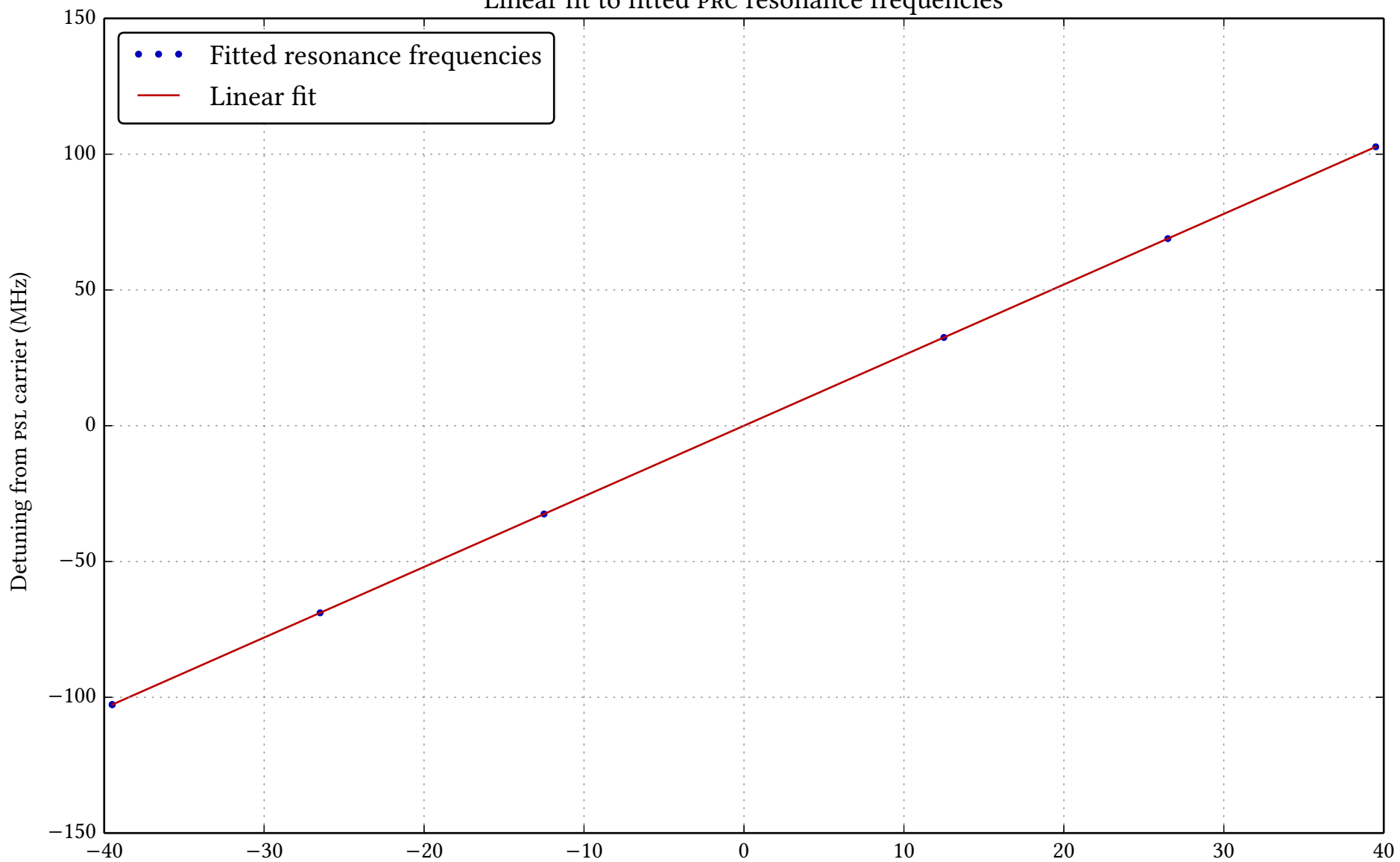
Linear fit to fitted PRC resonance frequencies
