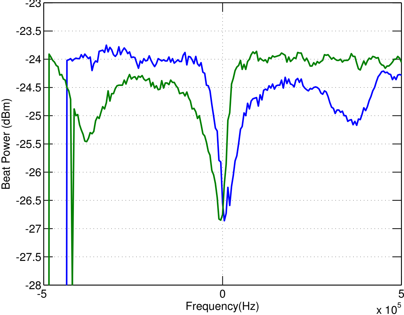
Reflected Beat Note Power from PRC
