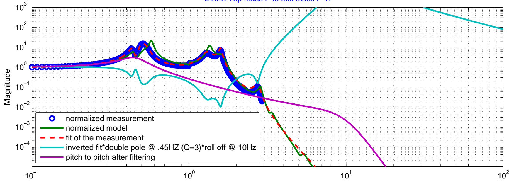
ETMX Top mass P to test mass P TF
