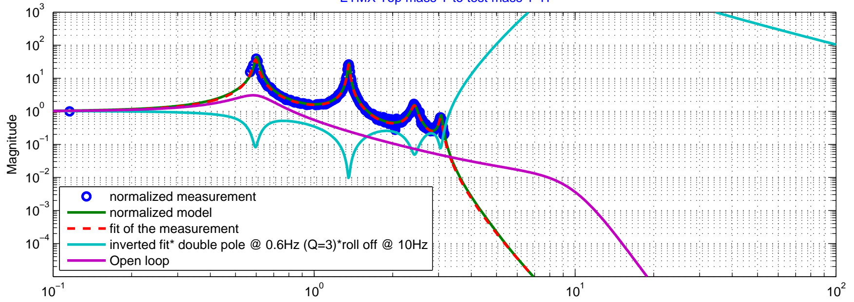
ETMX Top mass Y to test mass Y TF
