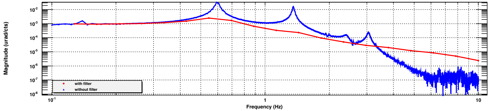
UIM YAW to test mass YAW transfer function
