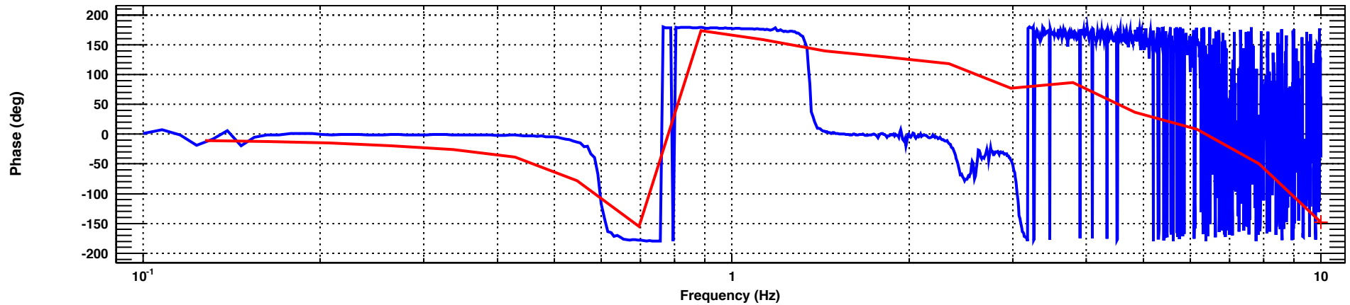
Transfer function
