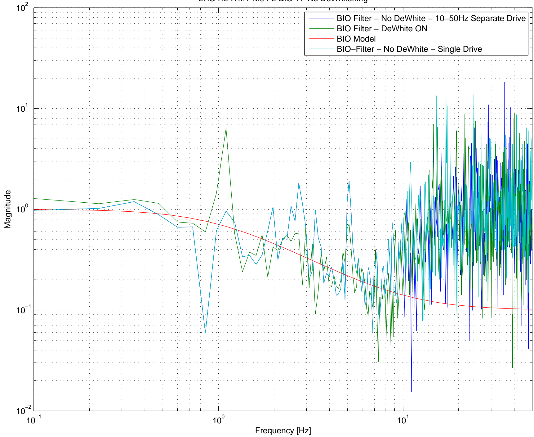
LHO H2 ITMY M0 F2 BIO TF No DeWhitening
