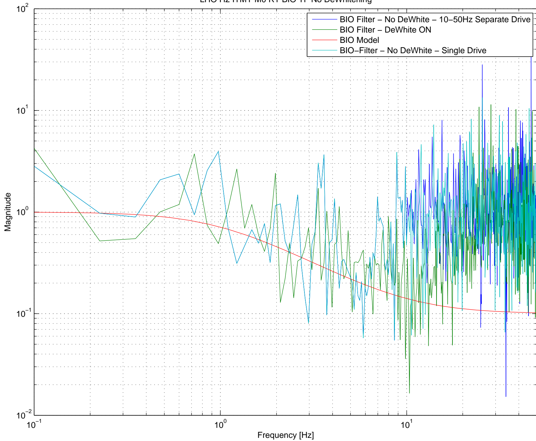
LHO H2 ITMY M0 RT BIO TF No DeWhitening
