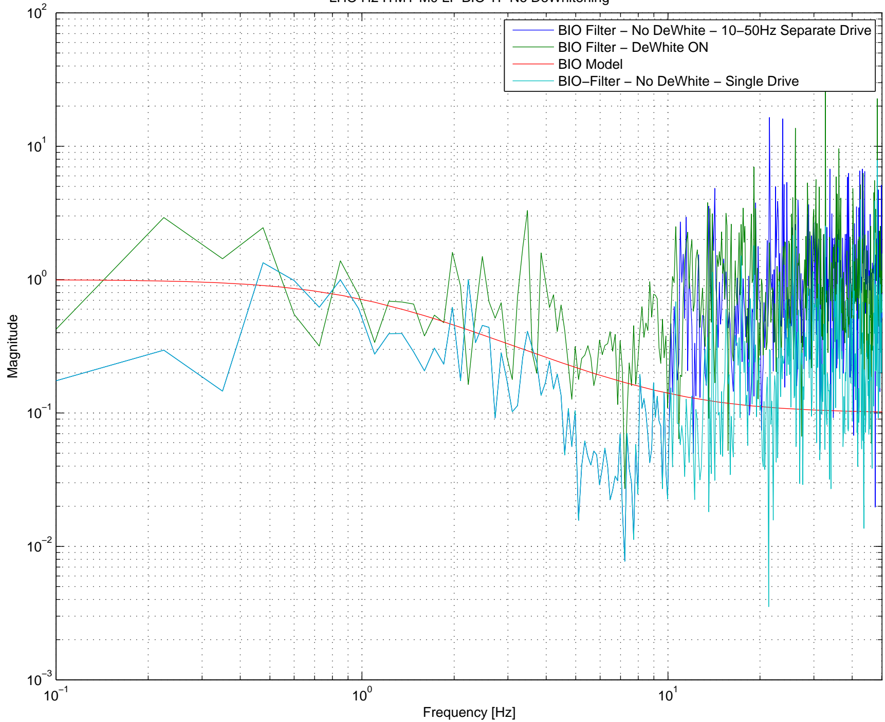
LHO H2 ITMY M0 LF BIO TF No DeWhitening
