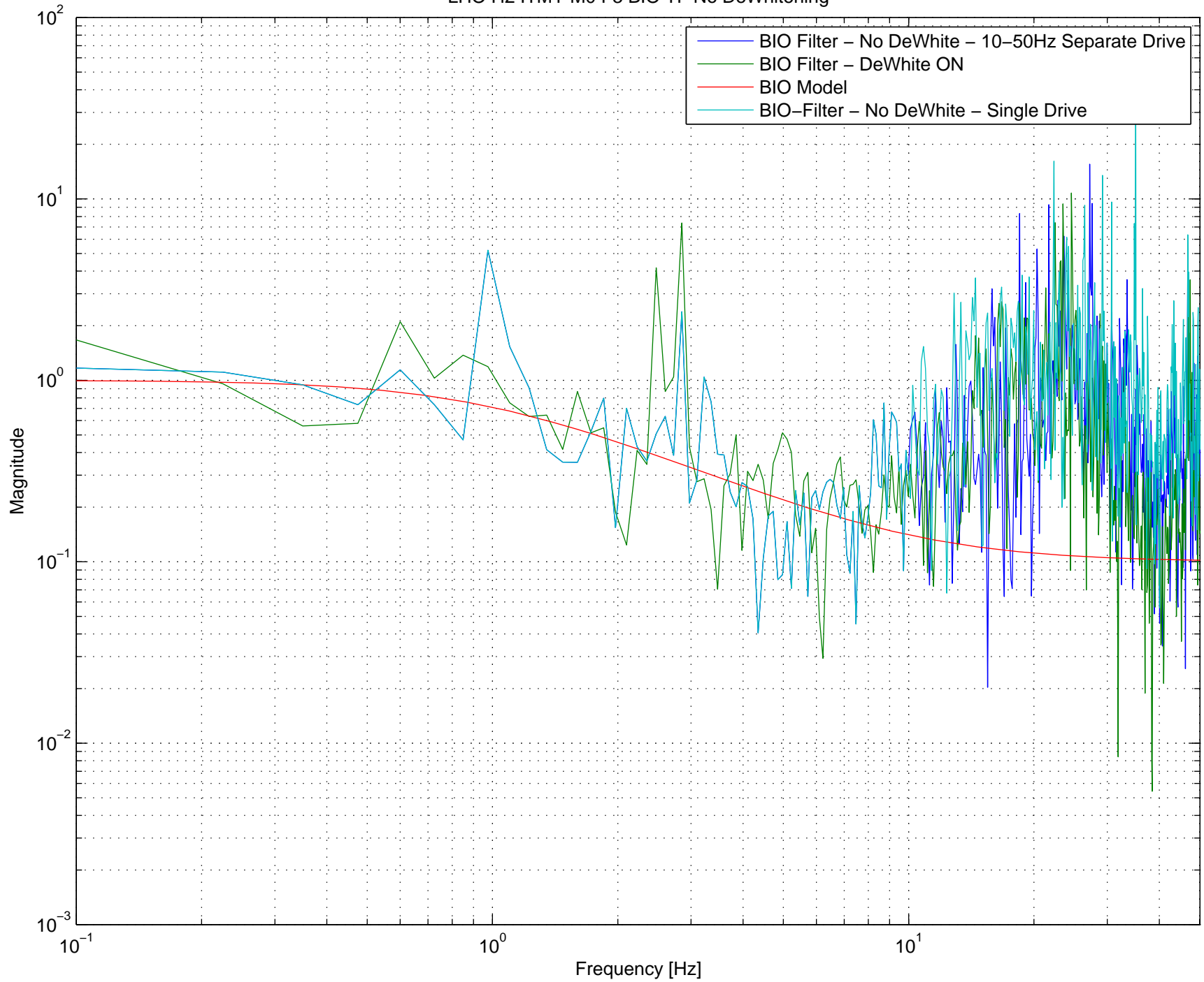
LHO H2 ITMY M0 F3 BIO TF No DeWhitening
