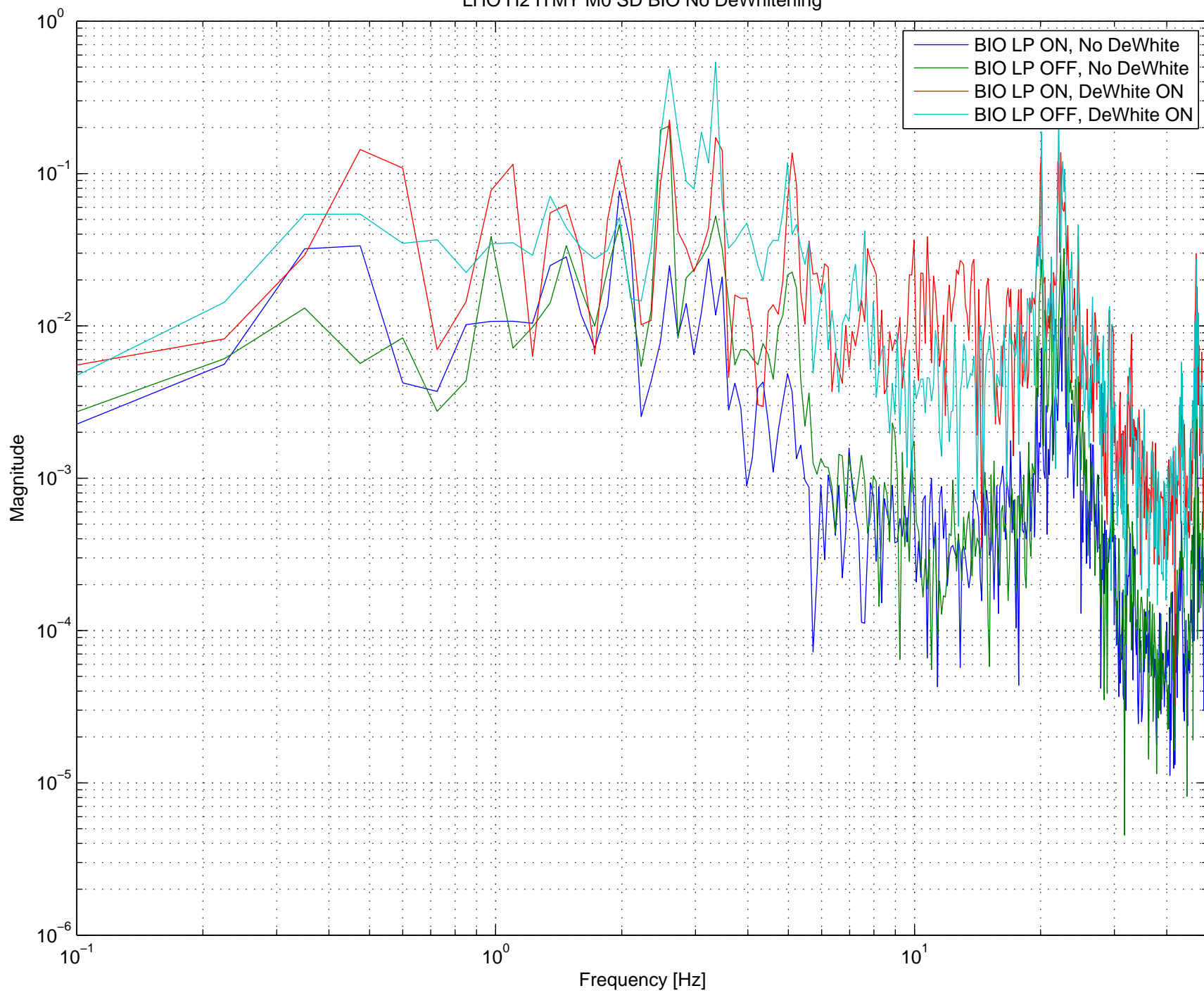
LHO H2 ITMY M0 SD BIO No DeWhitening
