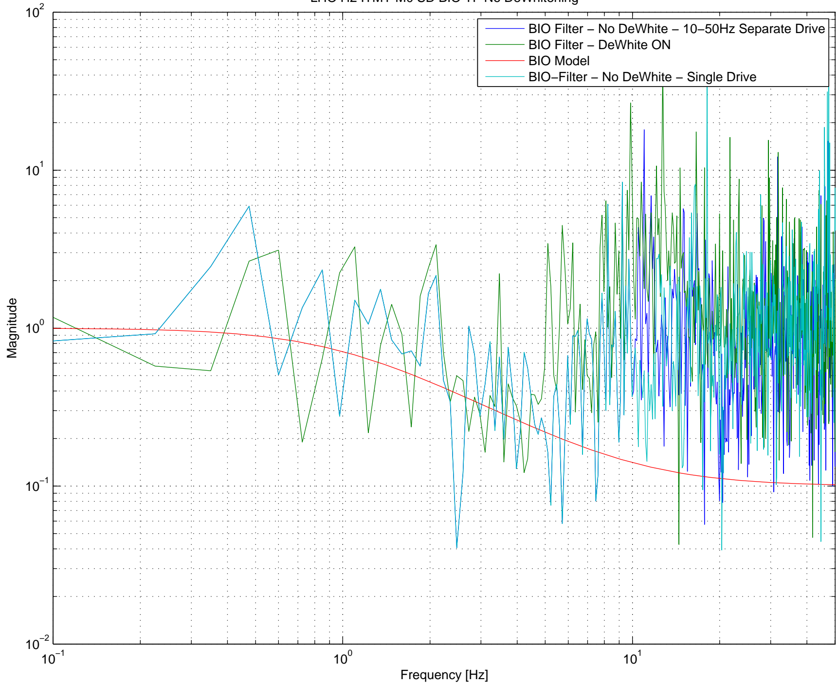
LHO H2 ITMY M0 SD BIO TF No DeWhitening
