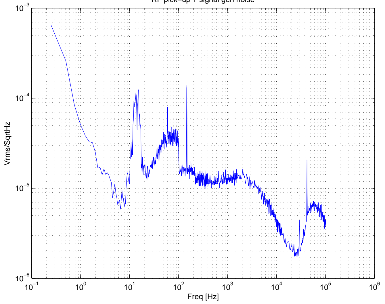
RF pick-up + signal gen noise
