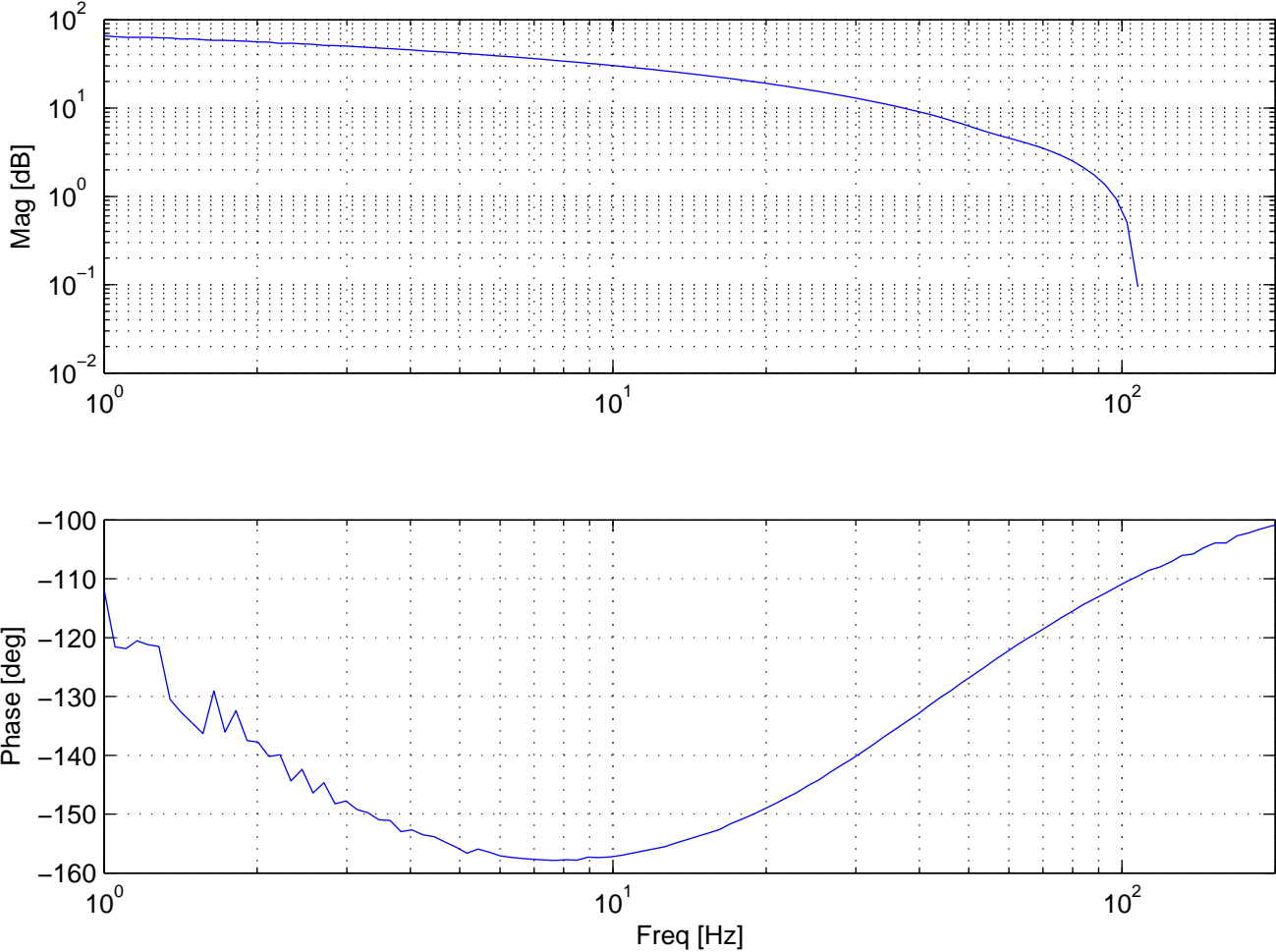
TF of modified COMM PLL Loop
