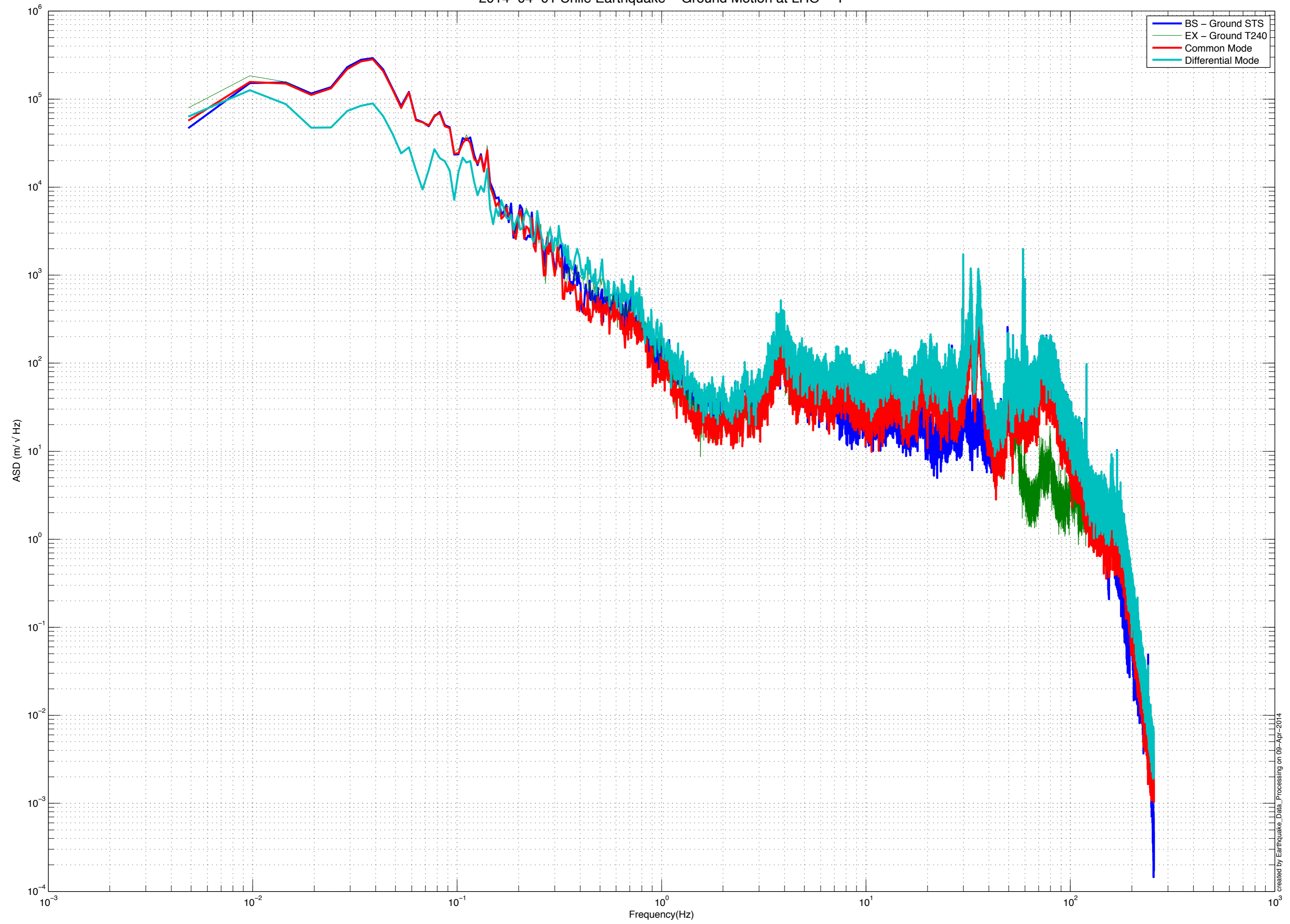
2014-04-01 Chile Earthquake – Ground Motion at LHO – Y
