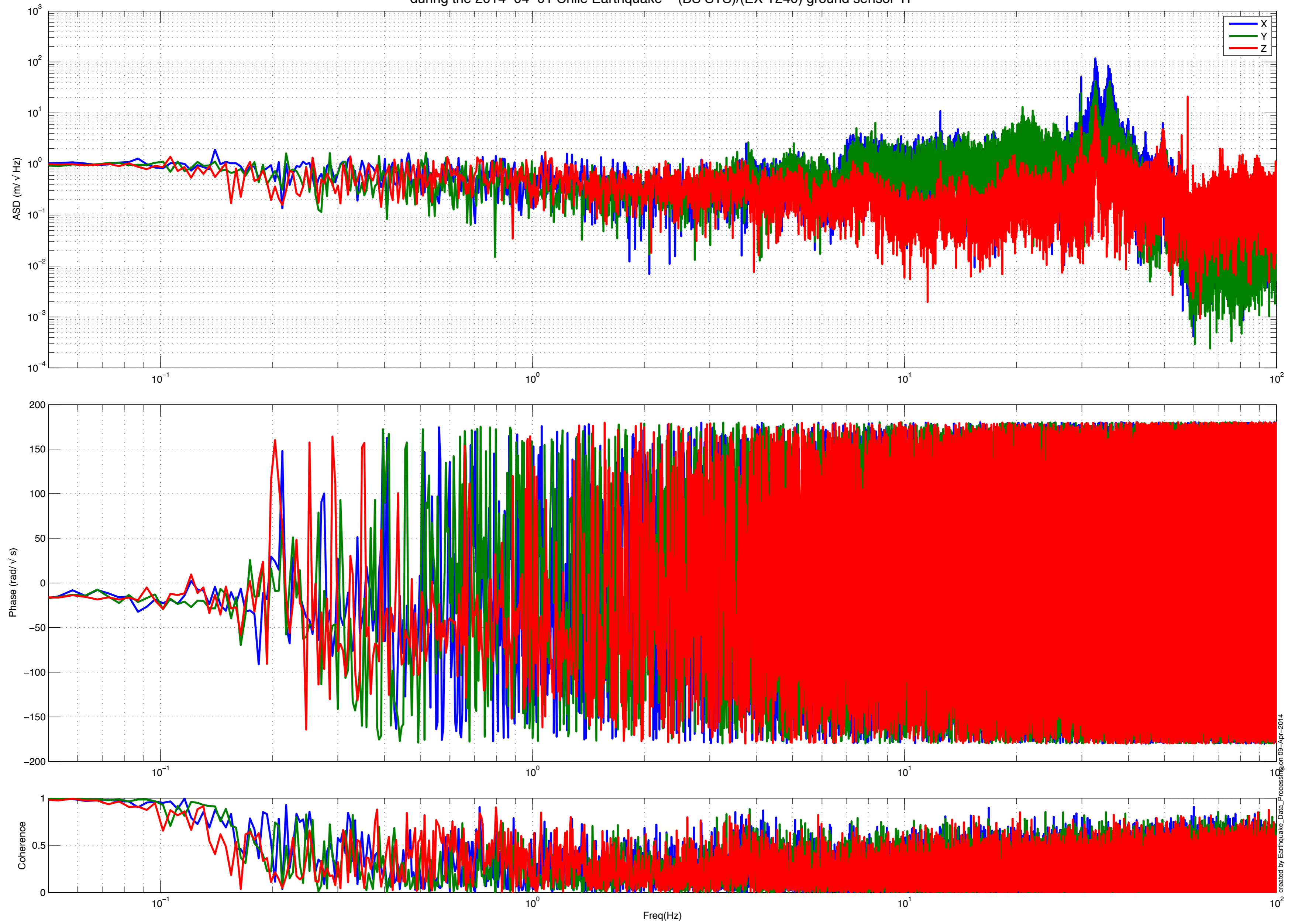
during the 2014-04-01 Chile Earthquake - (BS STS)/(EX T240) ground sensor TF
