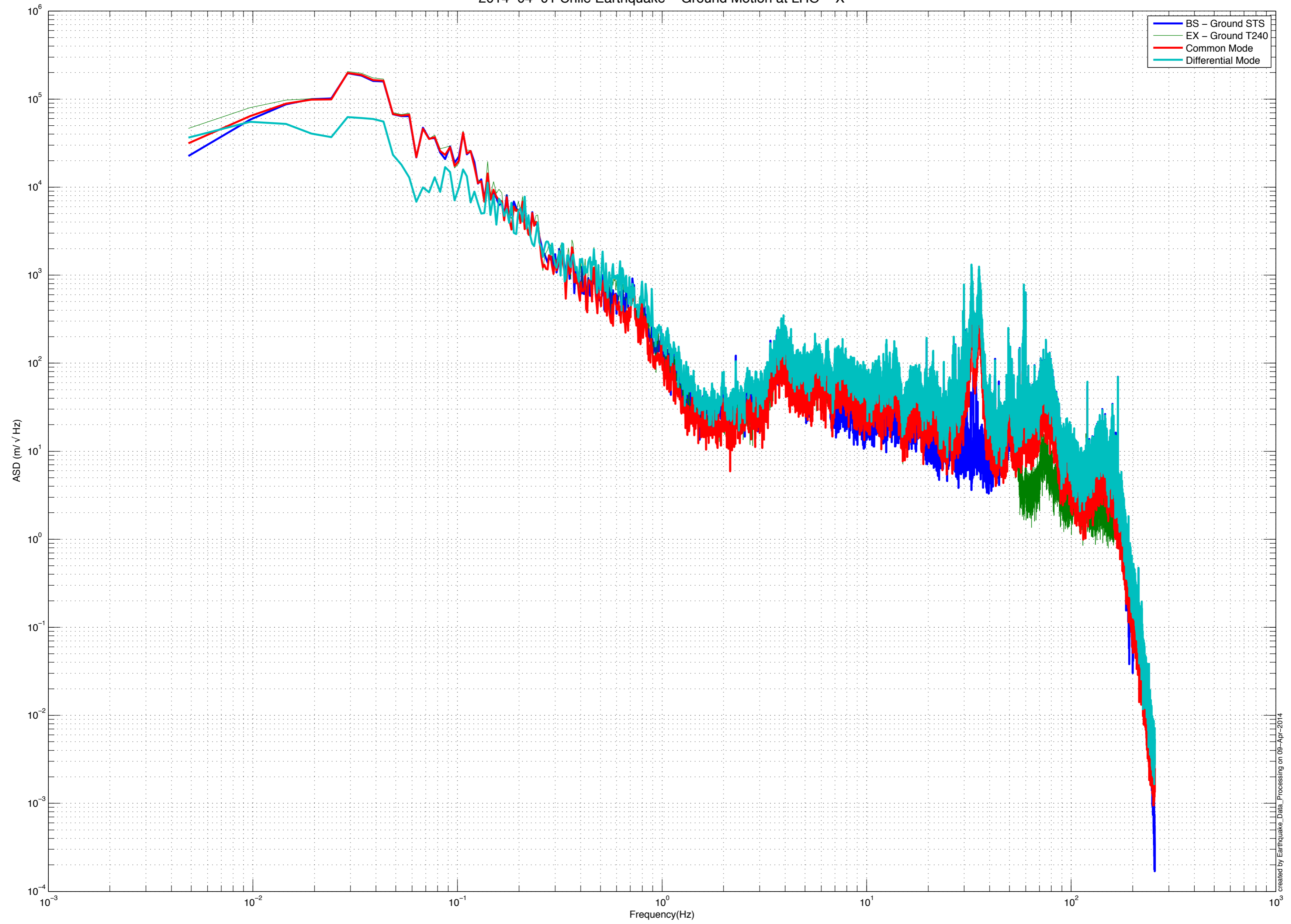
2014-04-01 Chile Earthquake – Ground Motion at LHO – X
