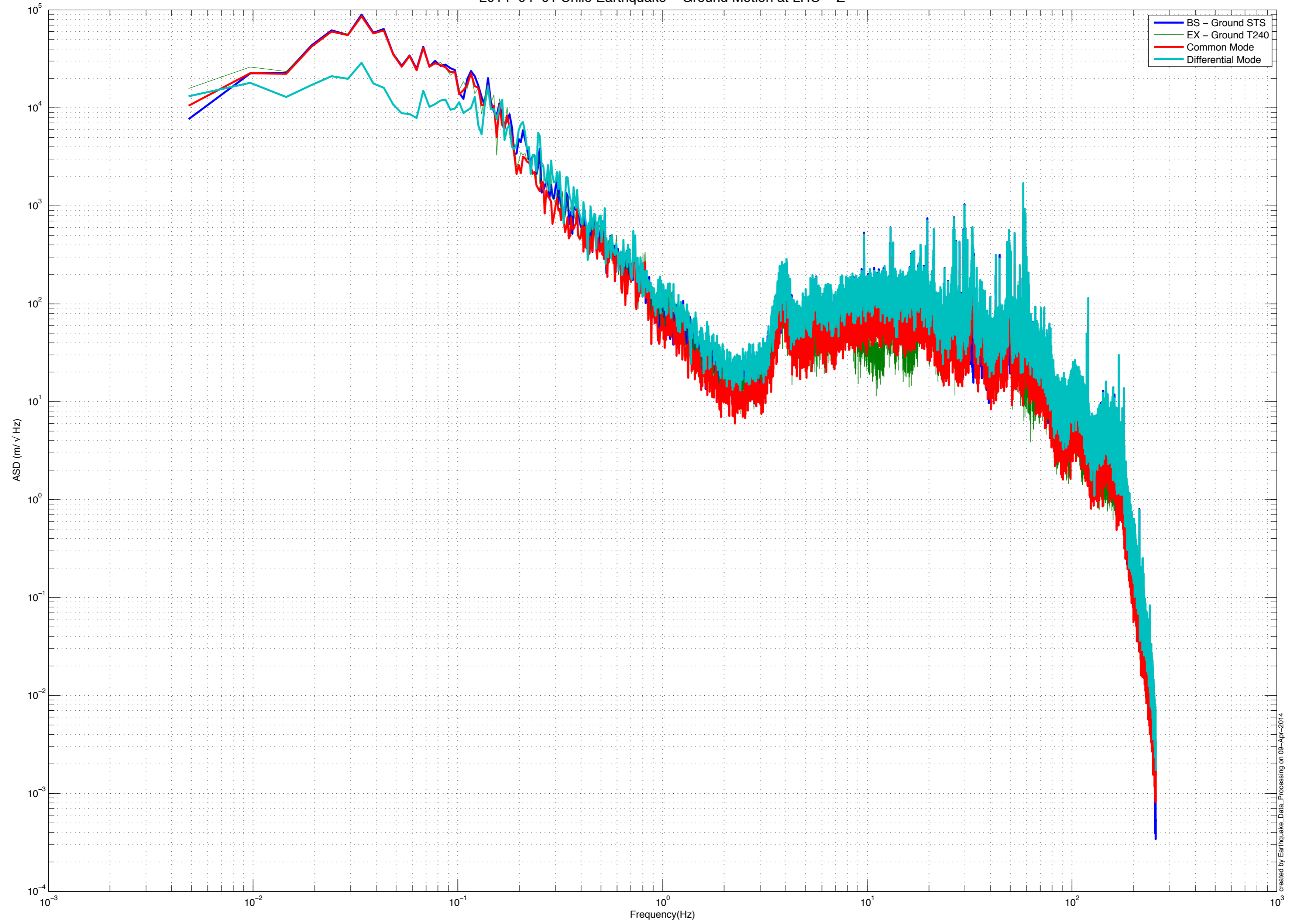
2014-04-01 Chile Earthquake – Ground Motion at LHO – Z
