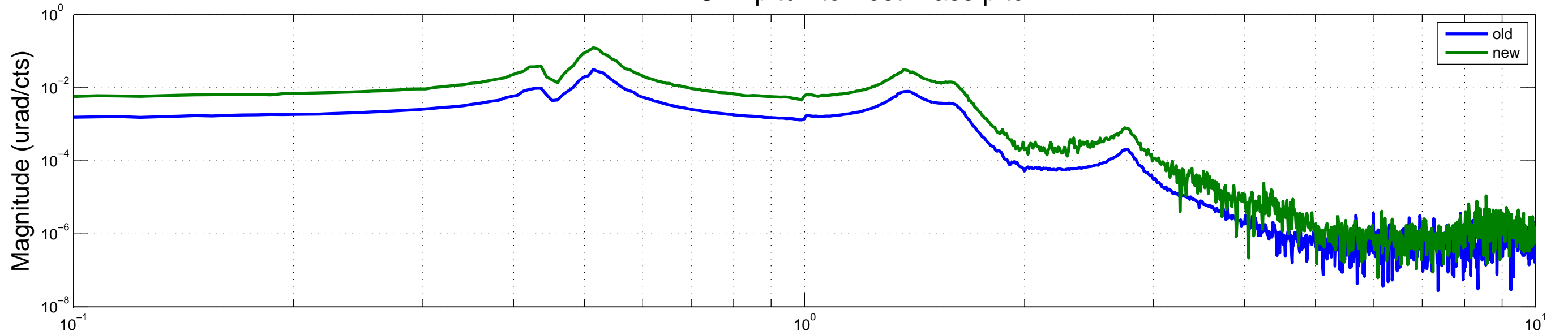
TF ETMY UIM pitch to Test Mass pitch
