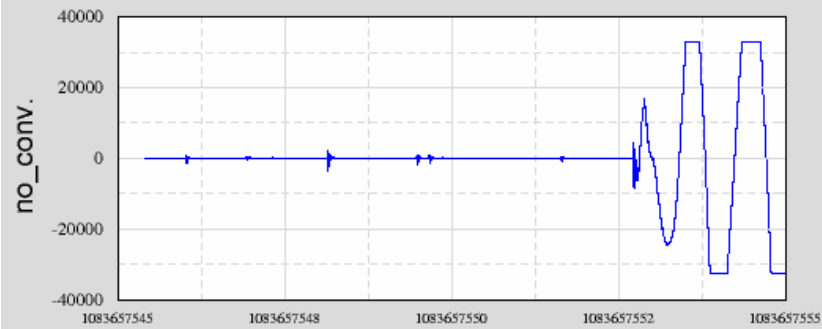
Ch 2: H1:HPI-ETMY_L4CINF_H1_IN1_DQ
