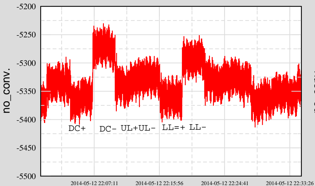
Ch 3: H1:SUS-ETMY_L3_OPLEV_SEG1_IN1_DQ
