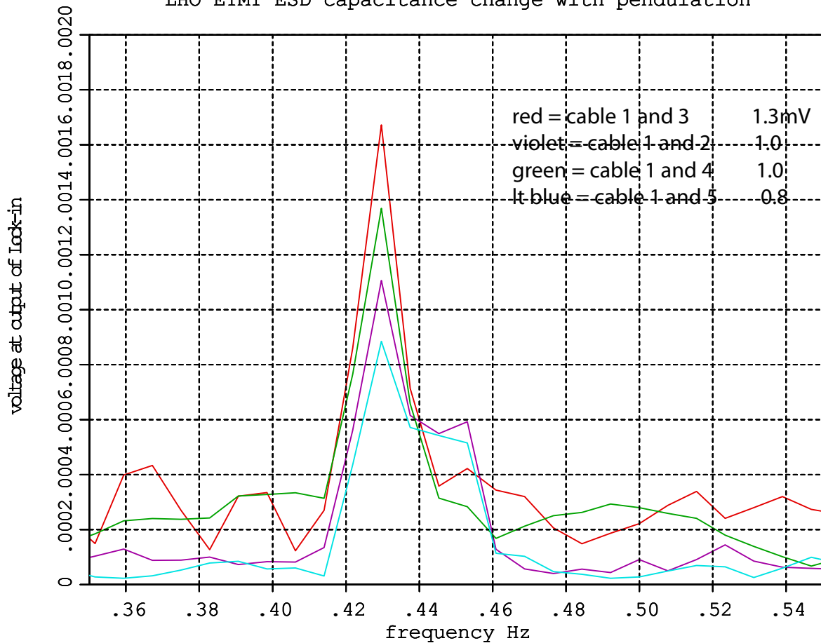
LHO ETMY ESD capacitance change with pendulation
