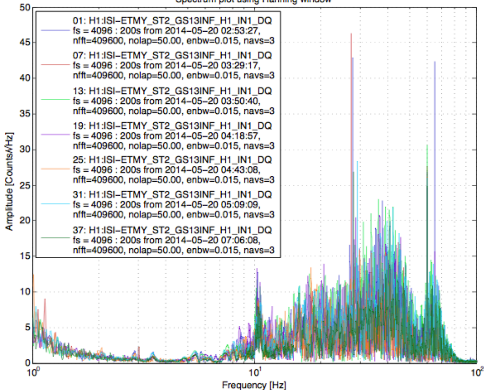
Spectrum plot using Hanning window
