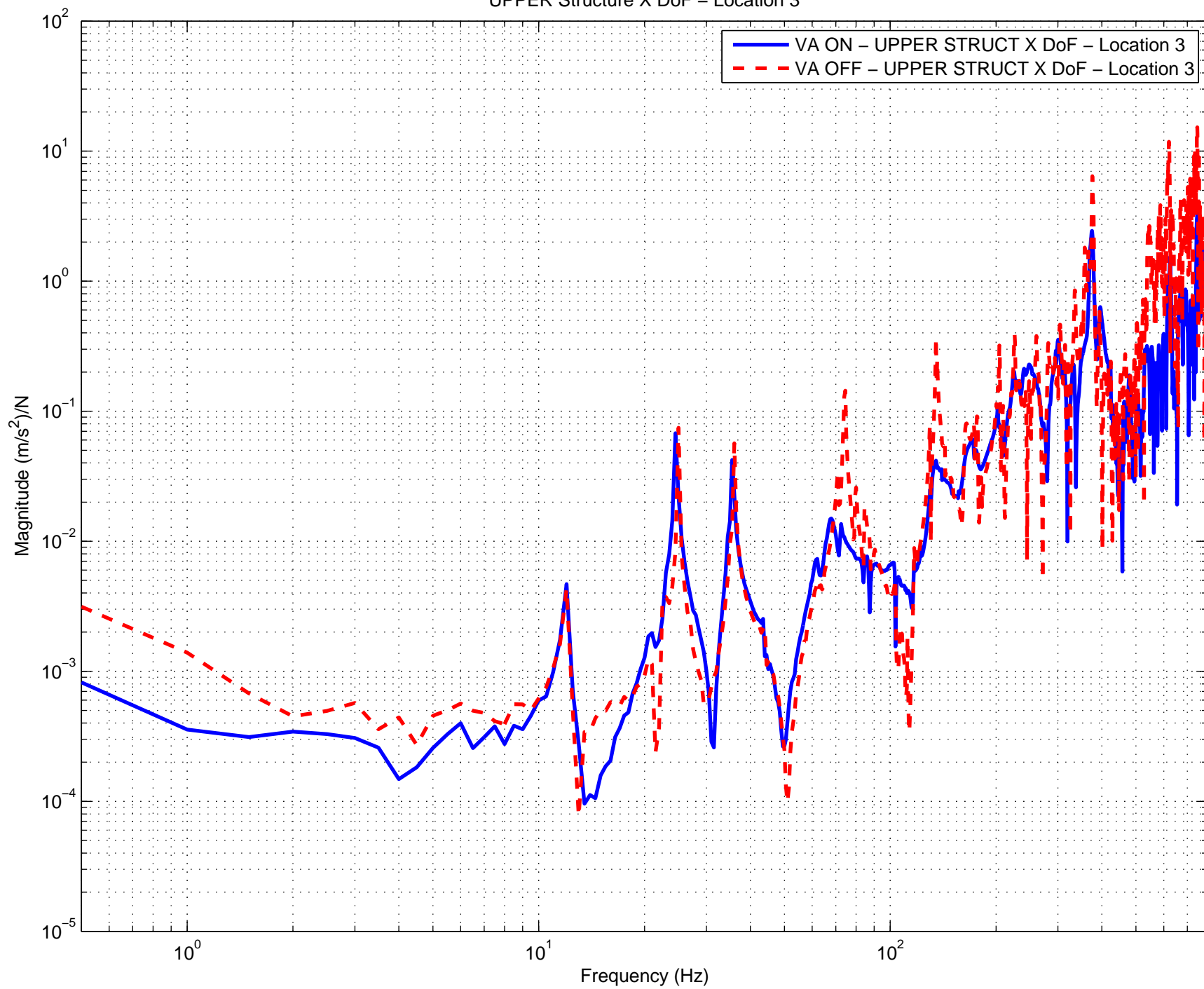
Vibration Absorbers H2 ITMY ON vs. OFF Comparison UPPER Structure X DoF – Location 3
