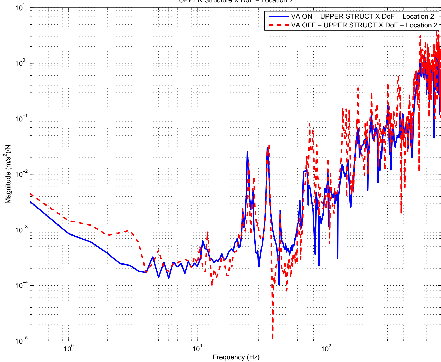
Vibration Absorbers H2 ITMY ON vs. OFF Comparison UPPER Structure X DoF – Location 2
