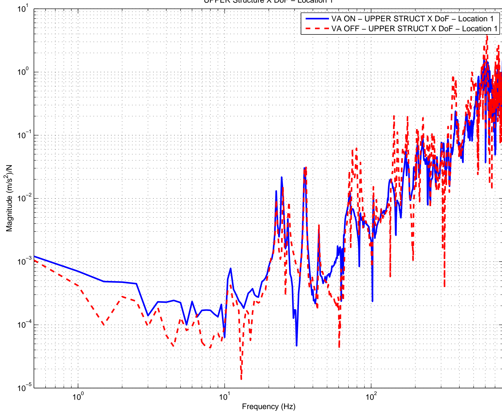
Vibration Absorbers H2 ITMY ON vs. OFF Comparison UPPER Structure X DoF – Location 1
