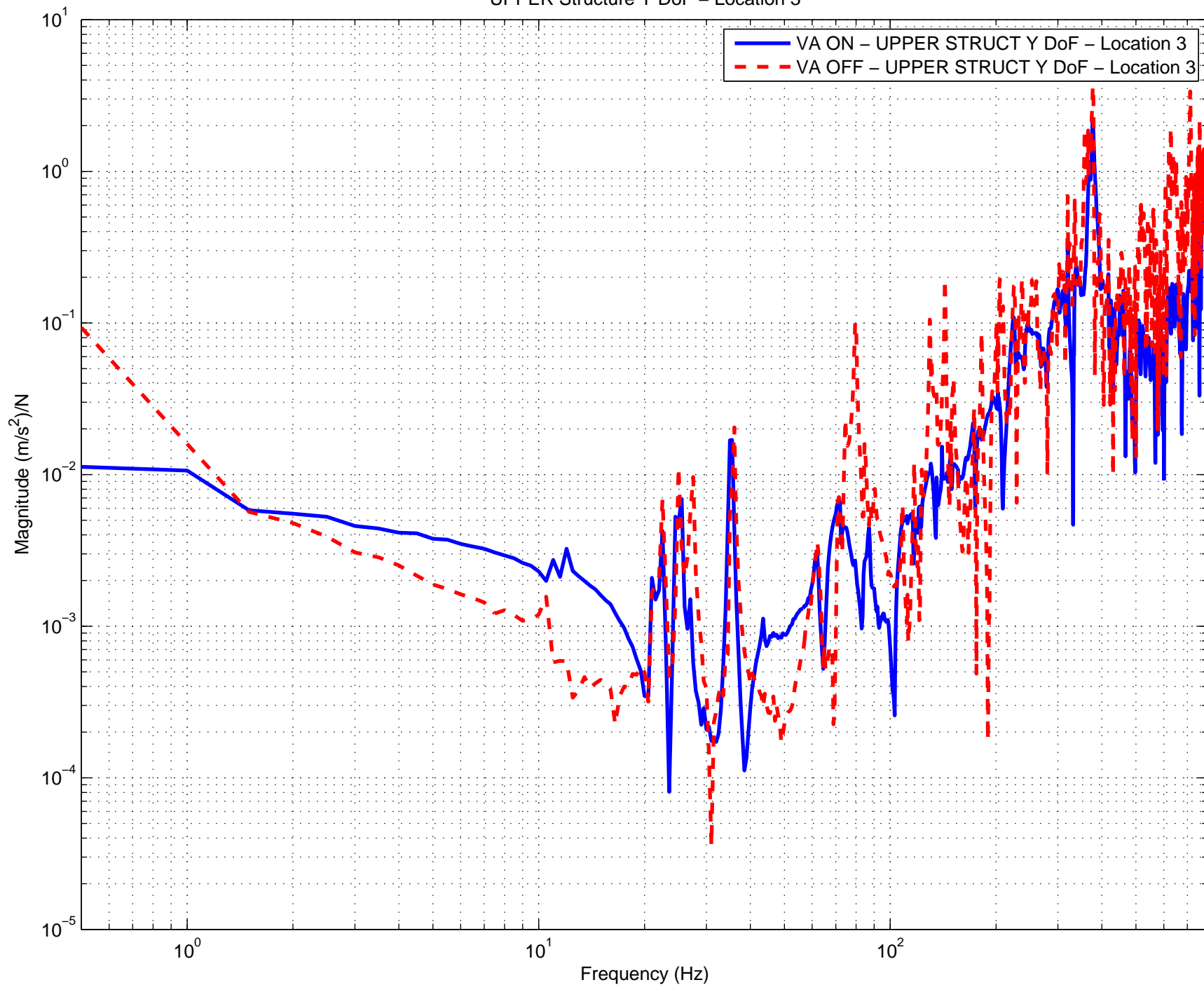
Vibration Absorbers H2 ITMY ON vs. OFF Comparison UPPER Structure Y DoF – Location 3
