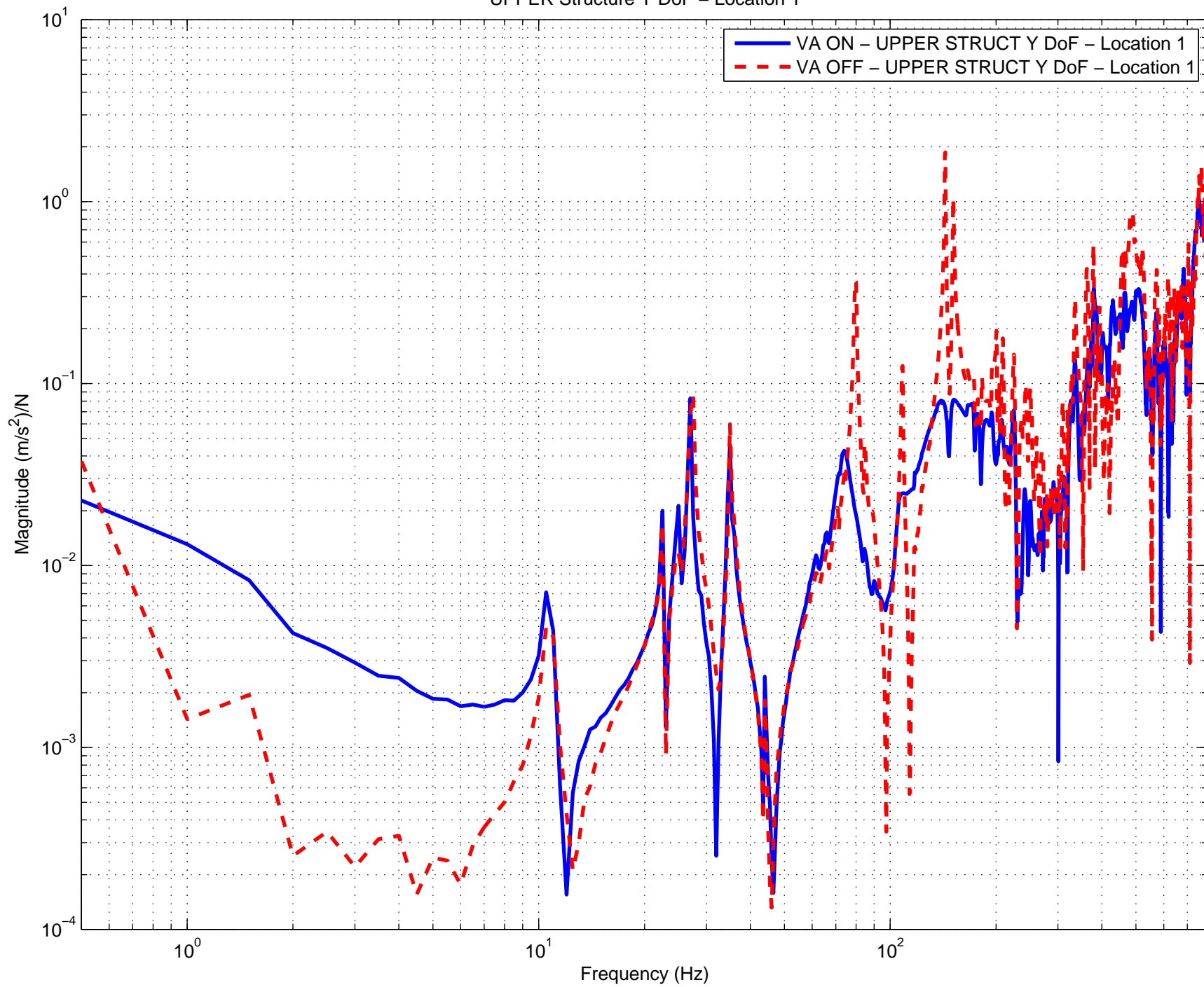
Vibration Absorbers H2 ITMY ON vs. OFF Comparison UPPER Structure Y DoF – Location 1
