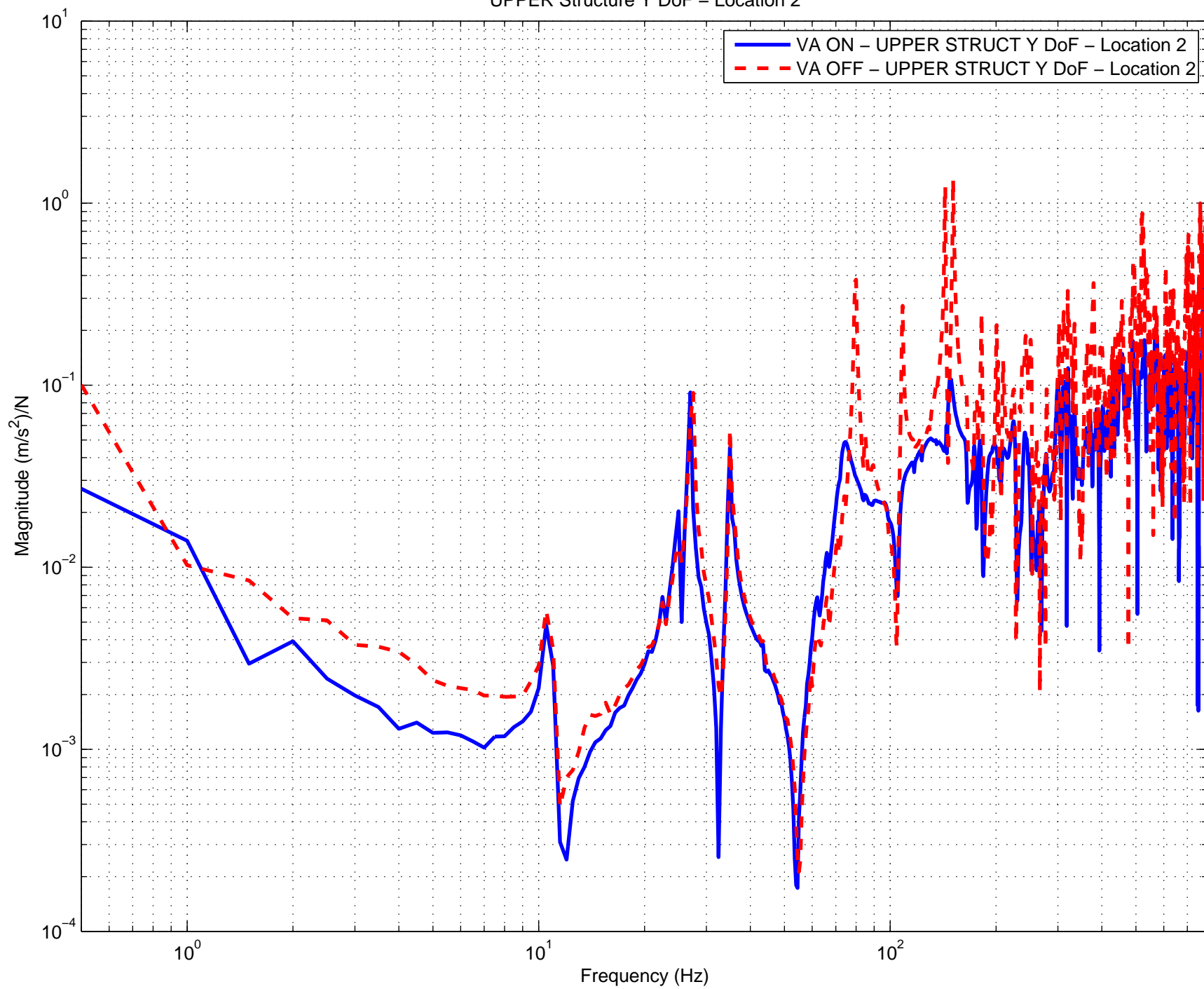
Vibration Absorbers H2 ITMY ON vs. OFF Comparison UPPER Structure Y DoF – Location 2
