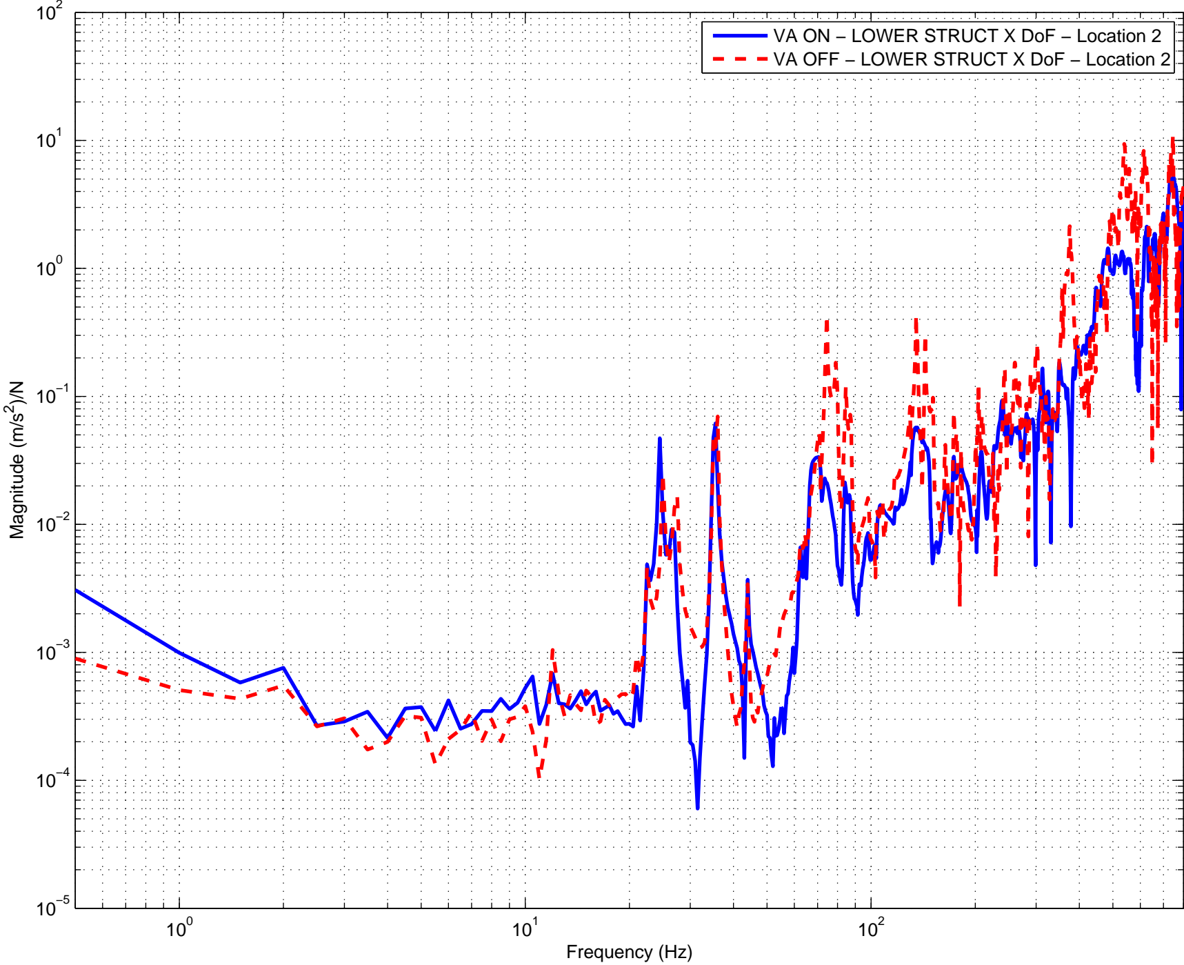
Vibration Absorbers H2 ITMY ON vs. OFF Comparison LOWER Structure X DoF – Location 2
