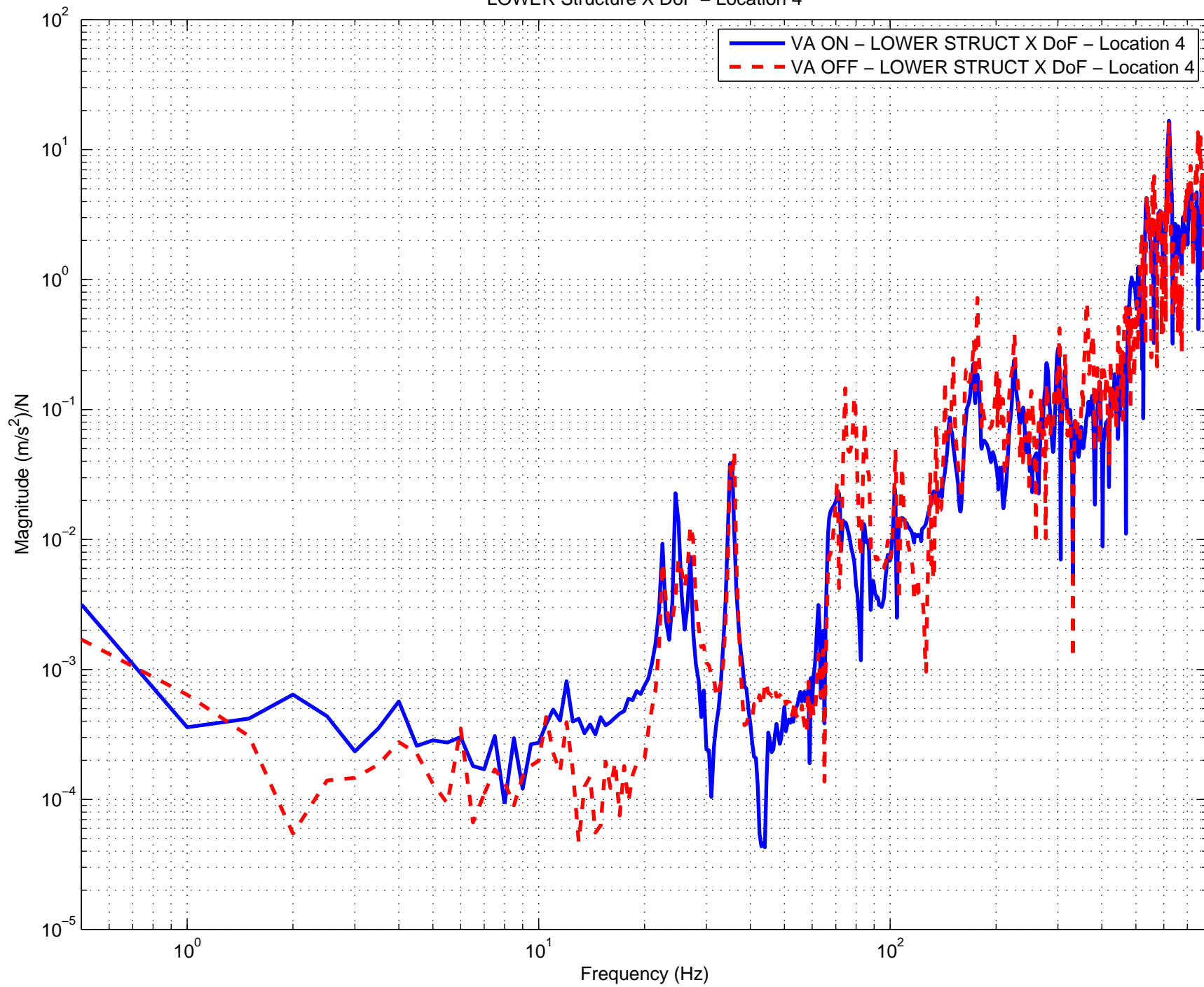
Vibration Absorbers H2 ITMY ON vs. OFF Comparison LOWER Structure X DoF – Location 4
