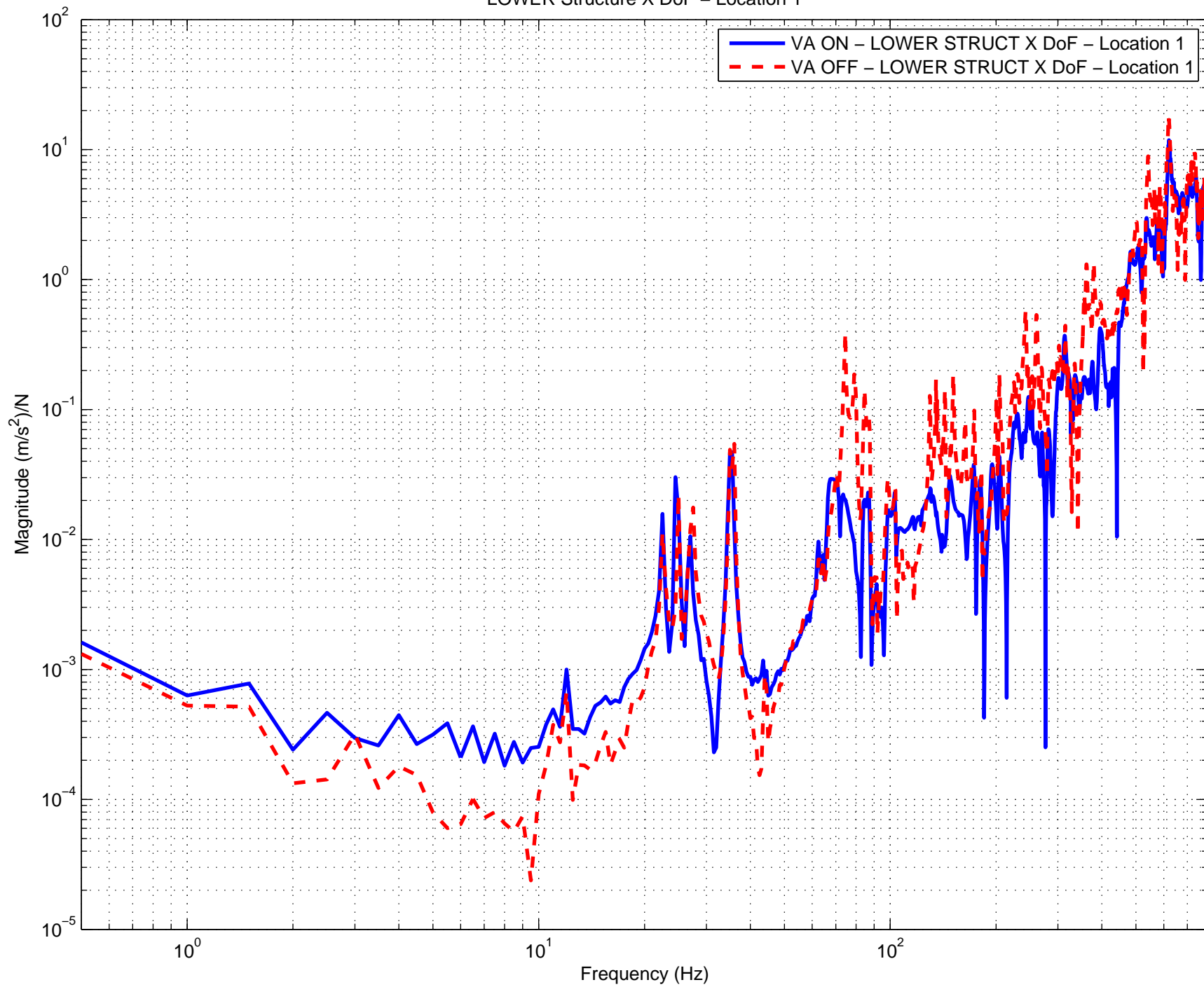
Vibration Absorbers H2 ITMY ON vs. OFF Comparison LOWER Structure X DoF – Location 1
