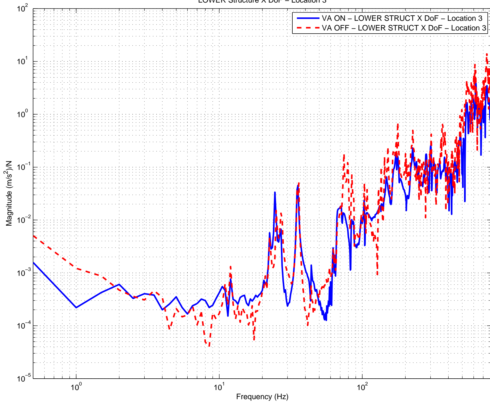
Vibration Absorbers H2 ITMY ON vs. OFF Comparison LOWER Structure X DoF – Location 3
