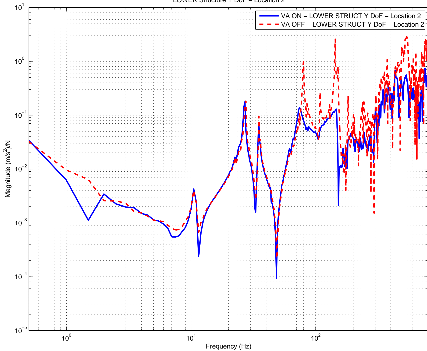
Vibration Absorbers H2 ITMY ON vs. OFF Comparison LOWER Structure Y DoF – Location 2
