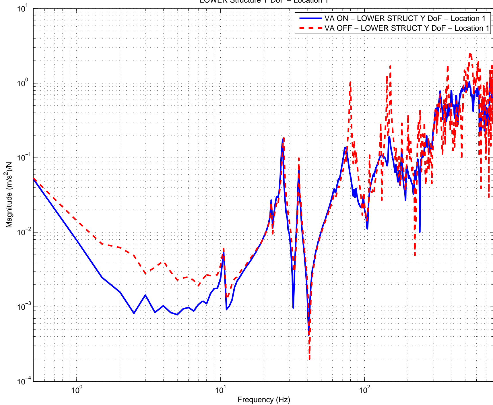
Vibration Absorbers H2 ITMY ON vs. OFF Comparison LOWER Structure Y DoF – Location 1
