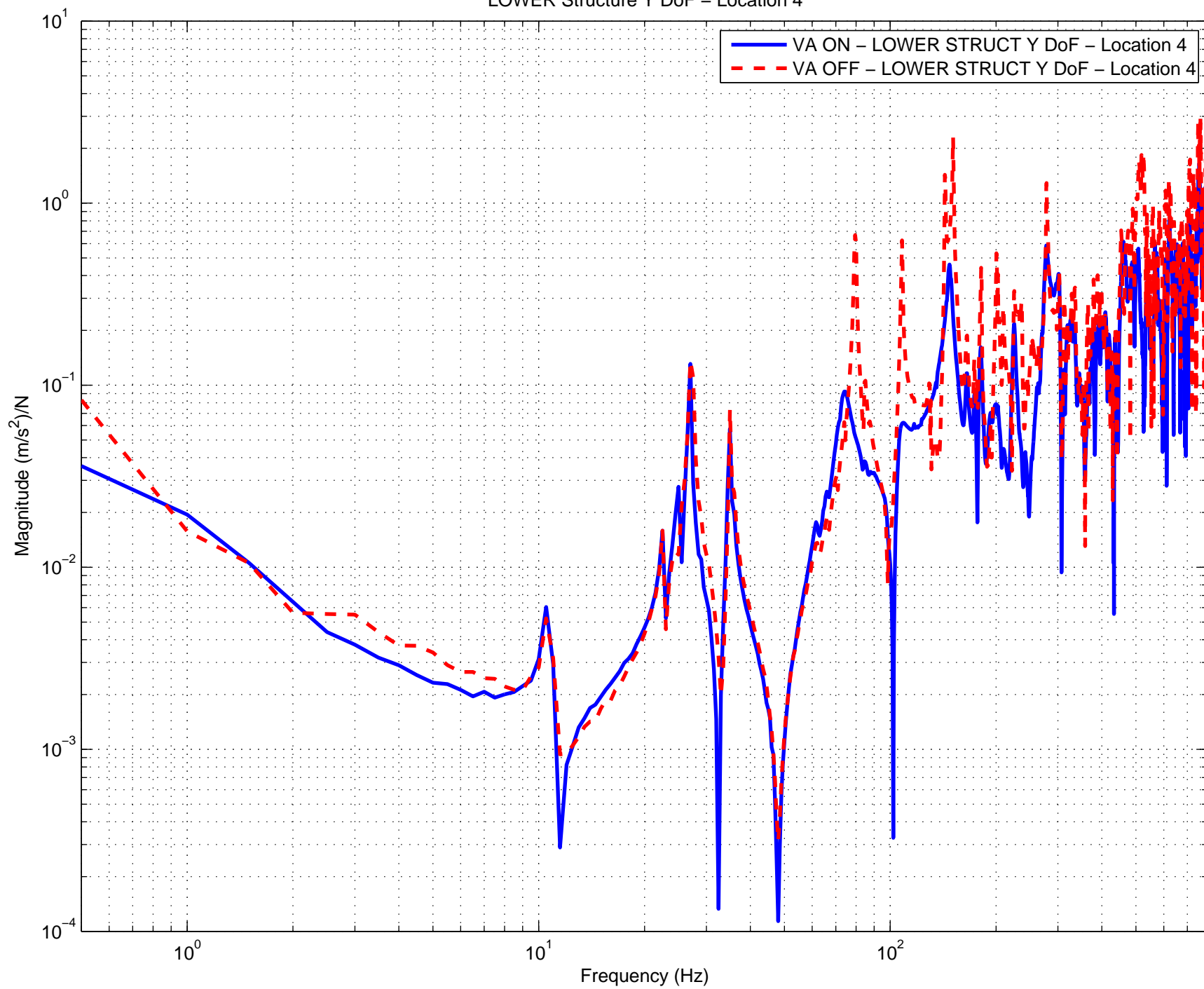
Vibration Absorbers H2 ITMY ON vs. OFF Comparison LOWER Structure Y DoF – Location 4
