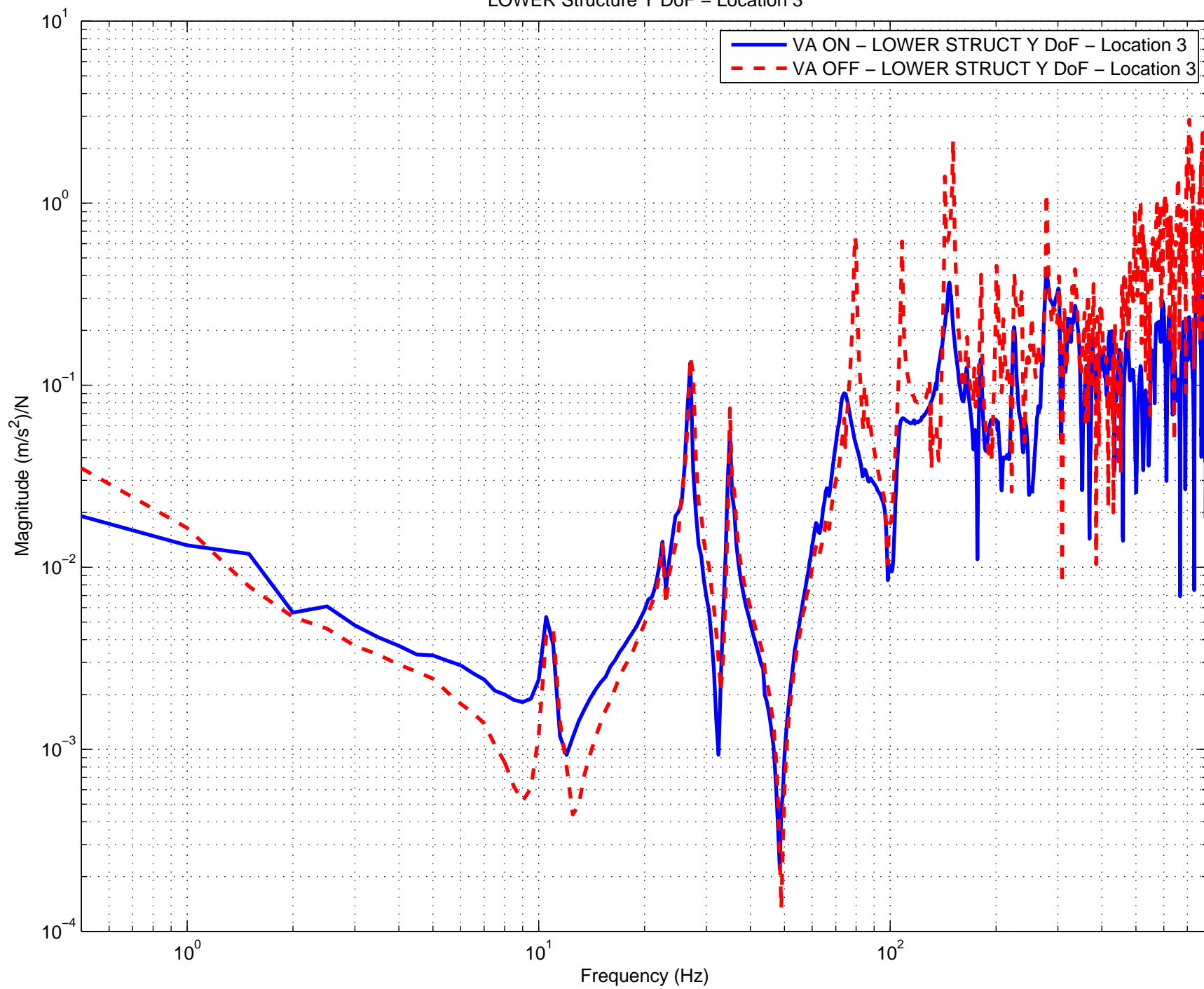
Vibration Absorbers H2 ITMY ON vs. OFF Comparison LOWER Structure Y DoF – Location 3
