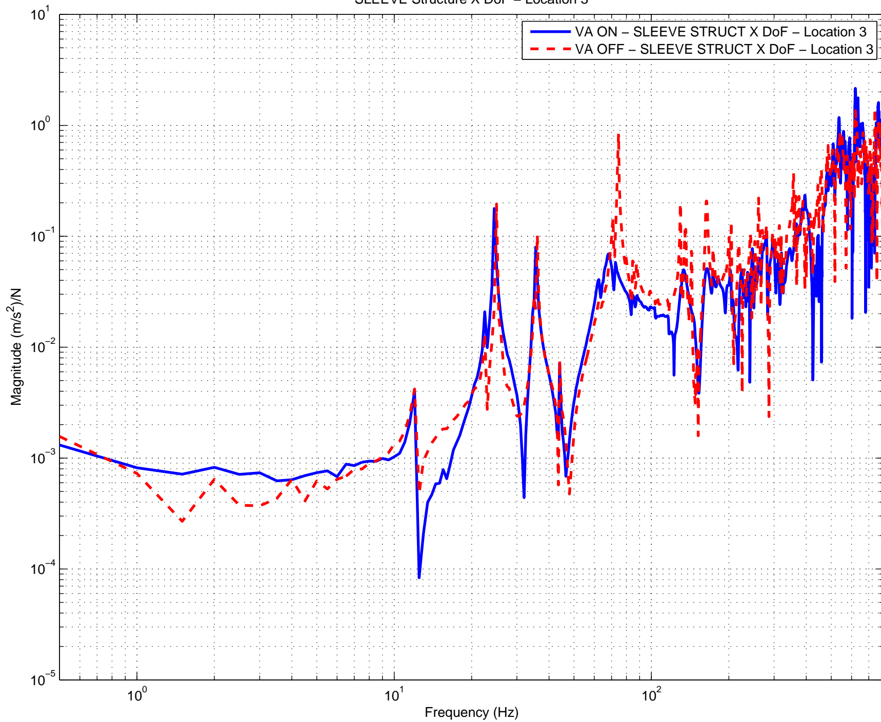
Vibration Absorbers H2 ITMY ON vs. OFF Comparison SLEEVE Structure X DoF – Location 3
