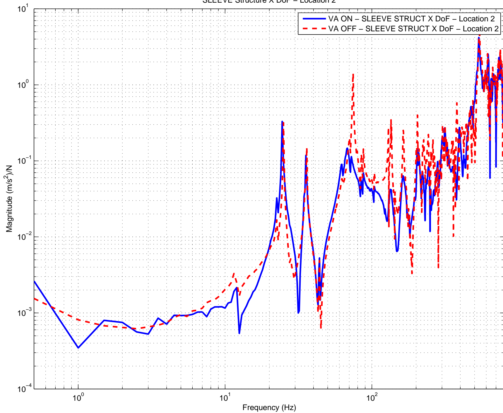
Vibration Absorbers H2 ITMY ON vs. OFF Comparison SLEEVE Structure X DoF – Location 2
