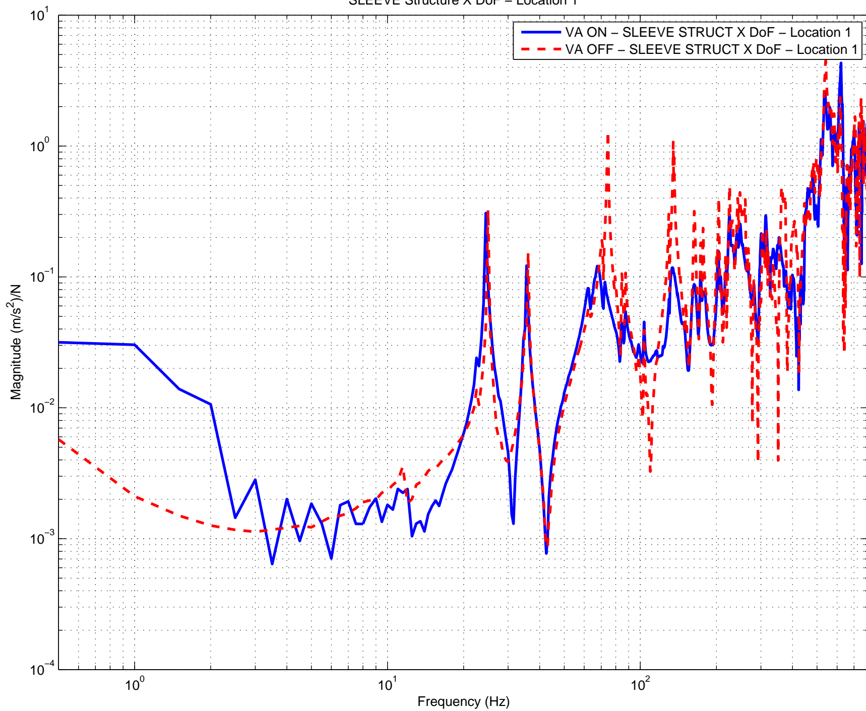
Vibration Absorbers H2 ITMY ON vs. OFF Comparison SLEEVE Structure X DoF – Location 1
