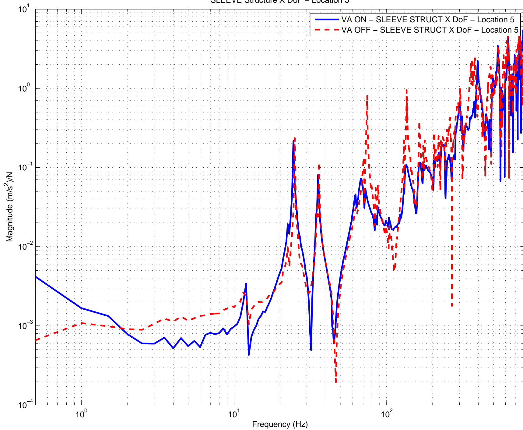
Vibration Absorbers H2 ITMY ON vs. OFF Comparison SLEEVE Structure X DoF – Location 5
