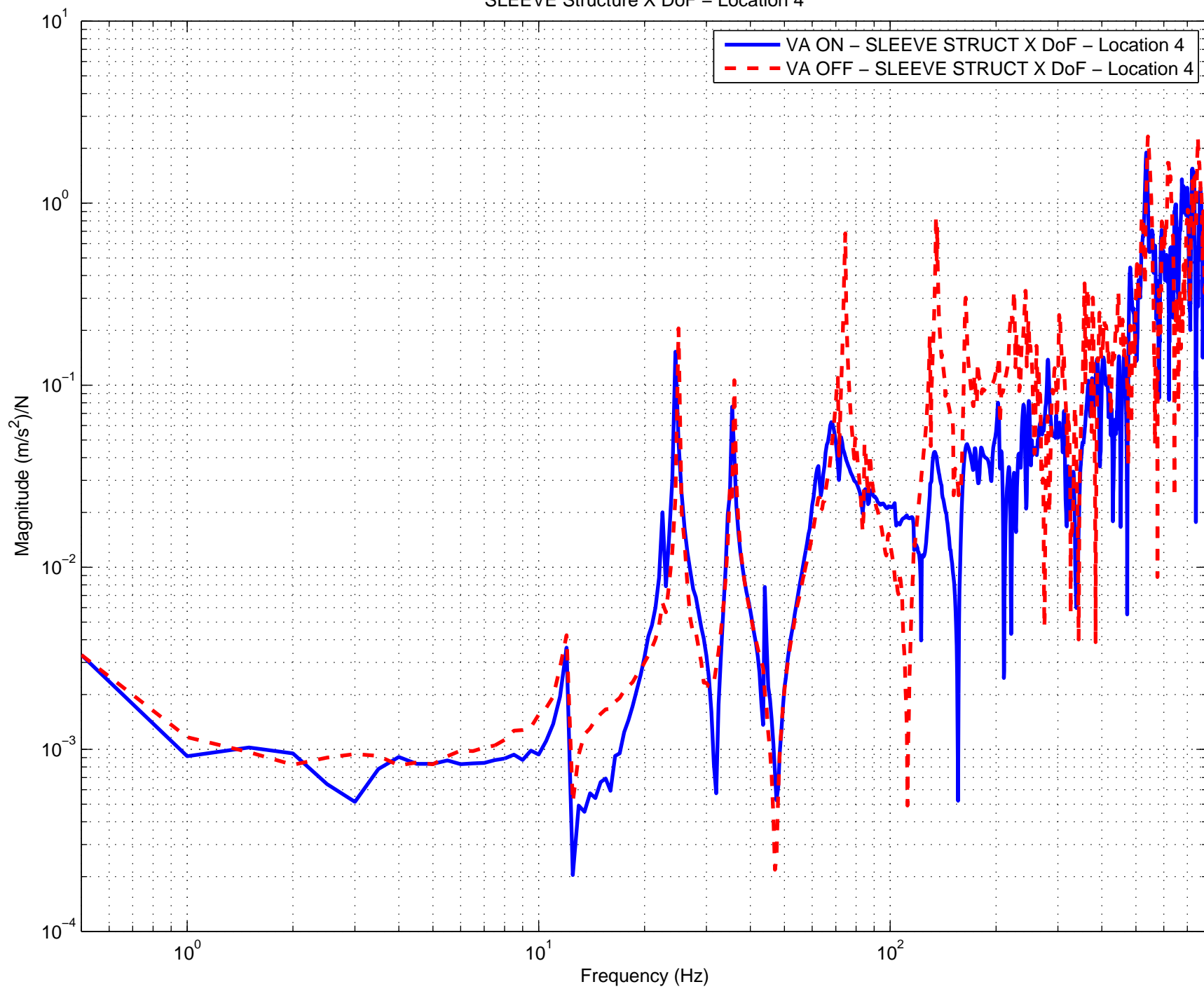
Vibration Absorbers H2 ITMY ON vs. OFF Comparison SLEEVE Structure X DoF – Location 4
