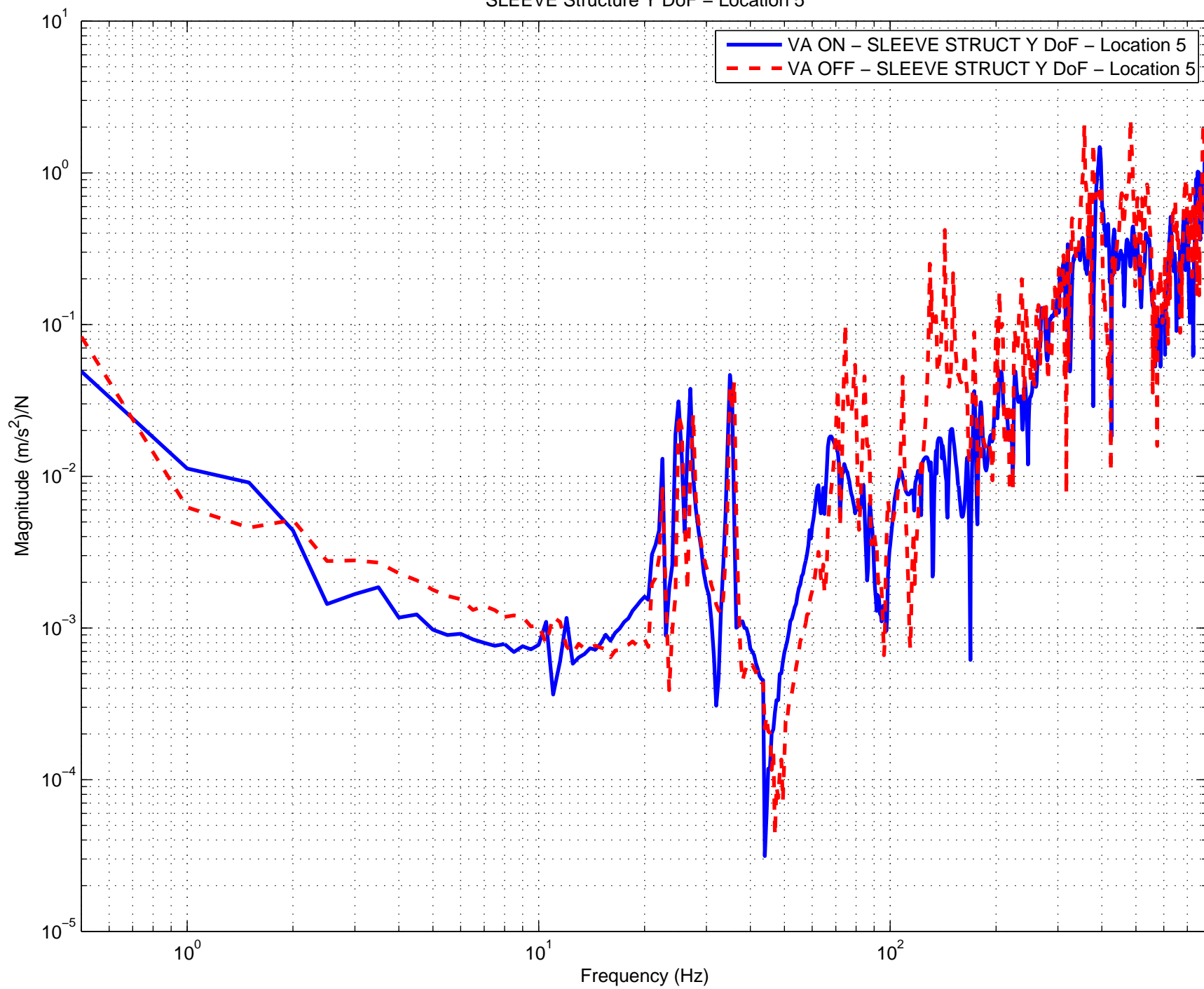
Vibration Absorbers H2 ITMY ON vs. OFF Comparison SLEEVE Structure Y DoF – Location 5
