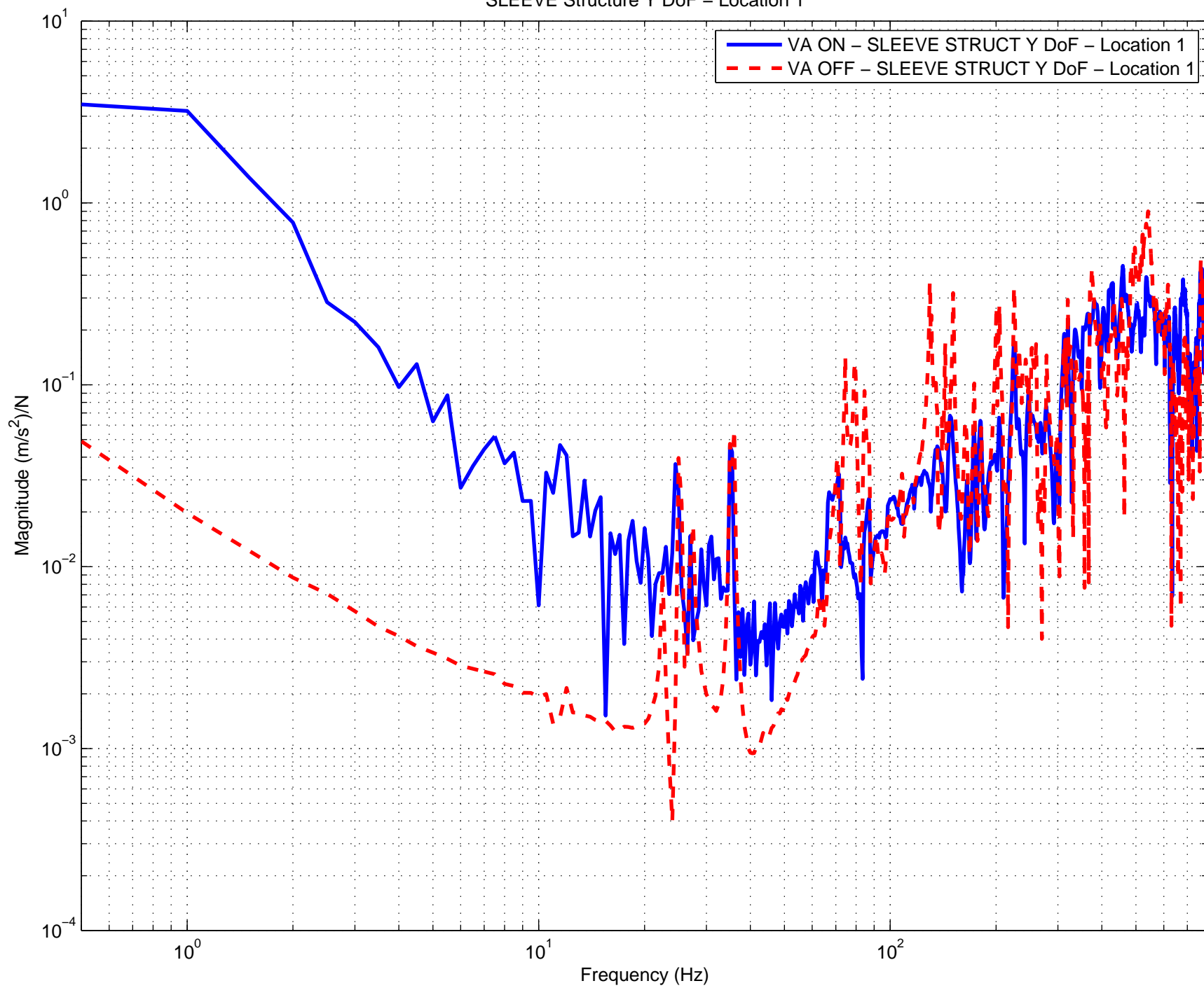
Vibration Absorbers H2 ITMY ON vs. OFF Comparison SLEEVE Structure Y DoF – Location 1
