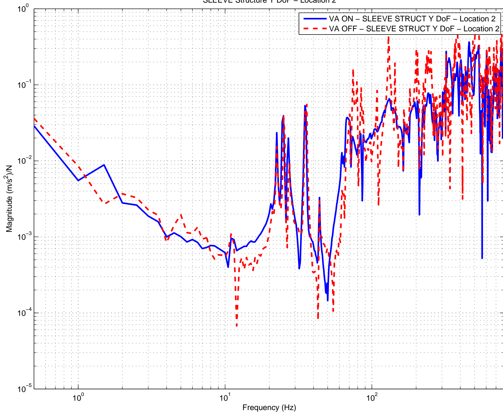
Vibration Absorbers H2 ITMY ON vs. OFF Comparison SLEEVE STRUCT Y DoF – Location 2
