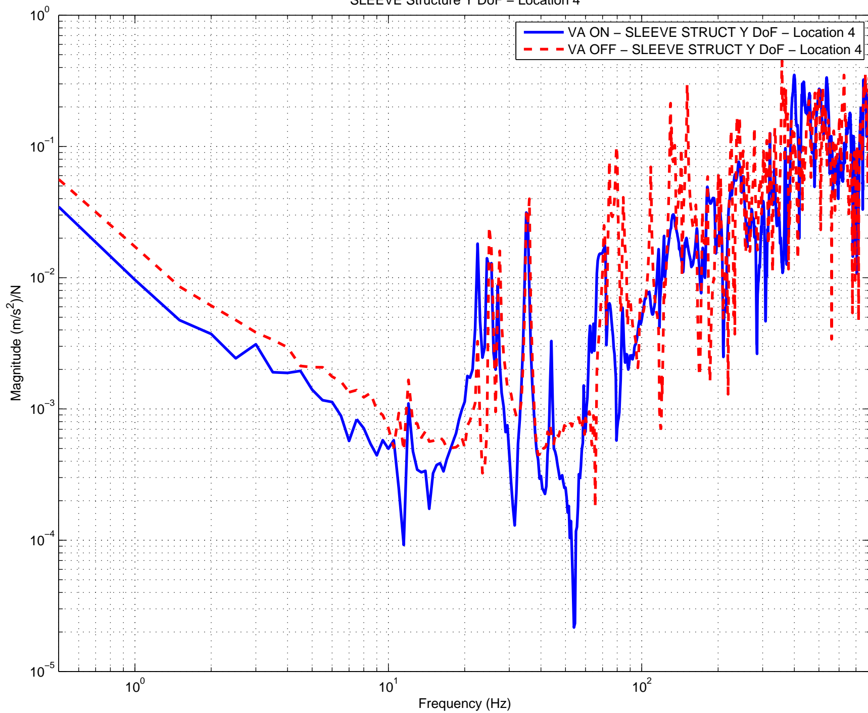
Vibration Absorbers H2 ITMY ON vs. OFF Comparison SLEEVE Structure Y DoF – Location 4
