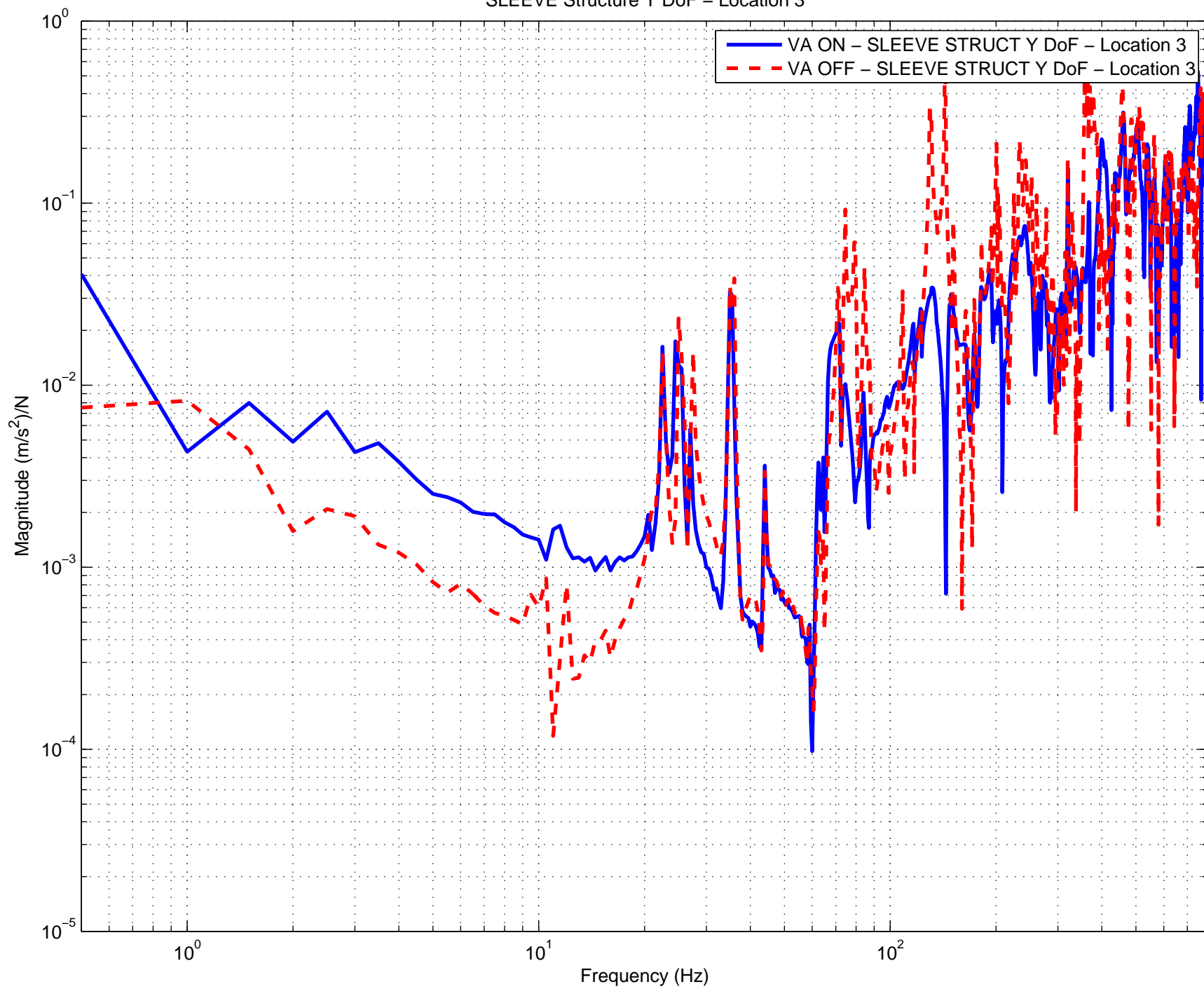
Vibration Absorbers H2 ITMY ON vs. OFF Comparison SLEEVE STRUCTURE Y DoF – Location 3
