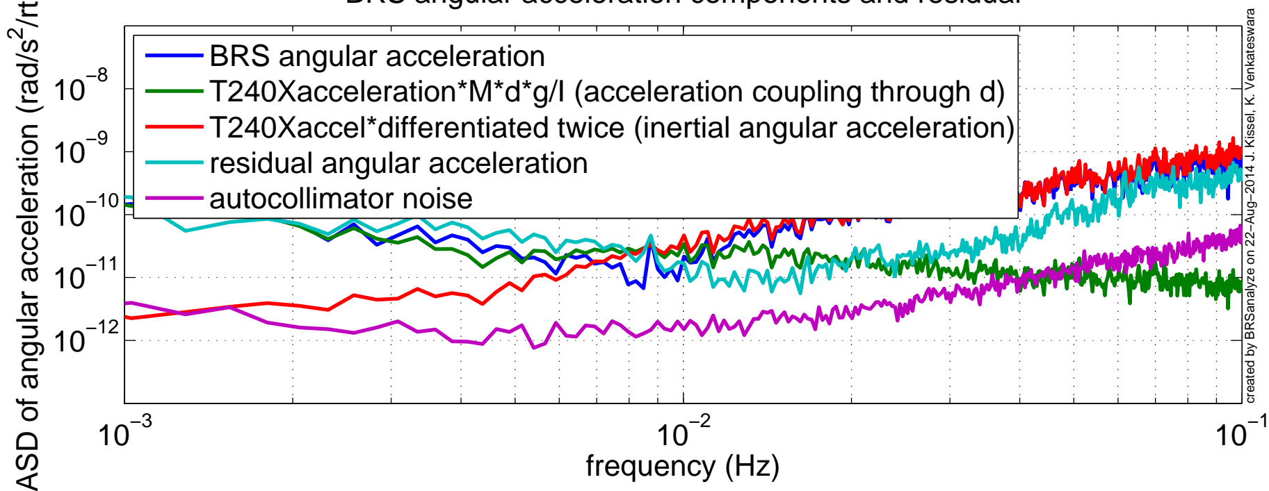
BRS angular acceleration components and residual
