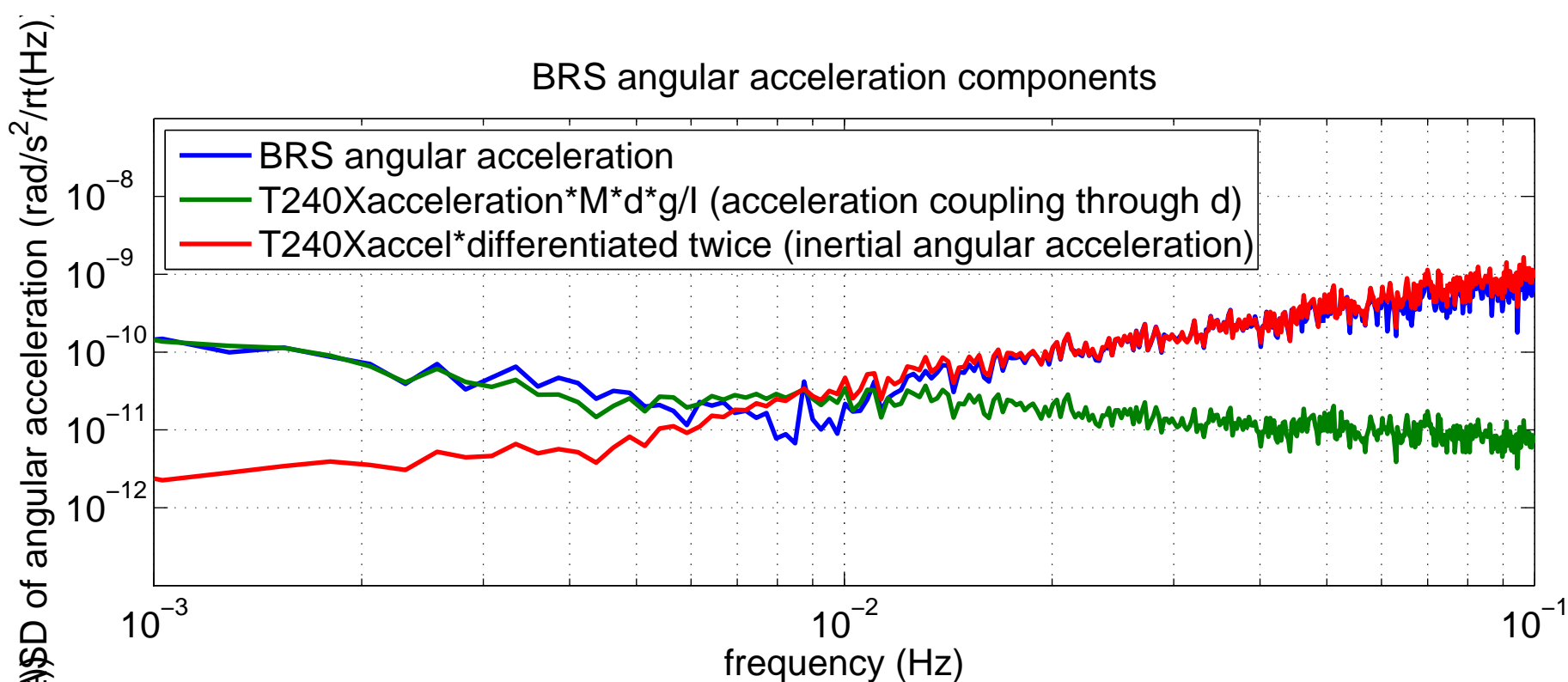
BRS angular acceleration components and residual
