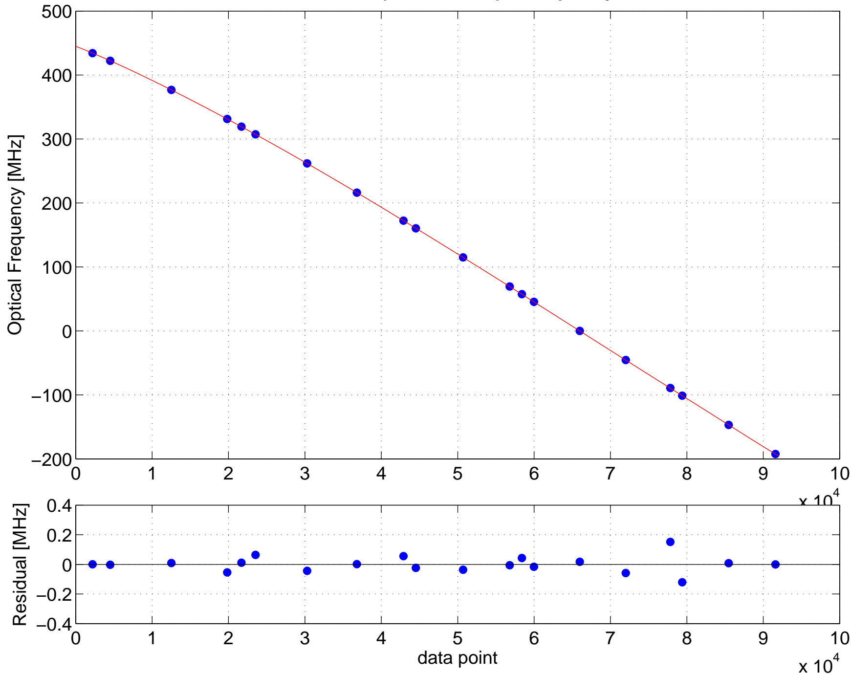
H1 OMC mode scan (ALOG:13660) ~ Frequency Calibration
