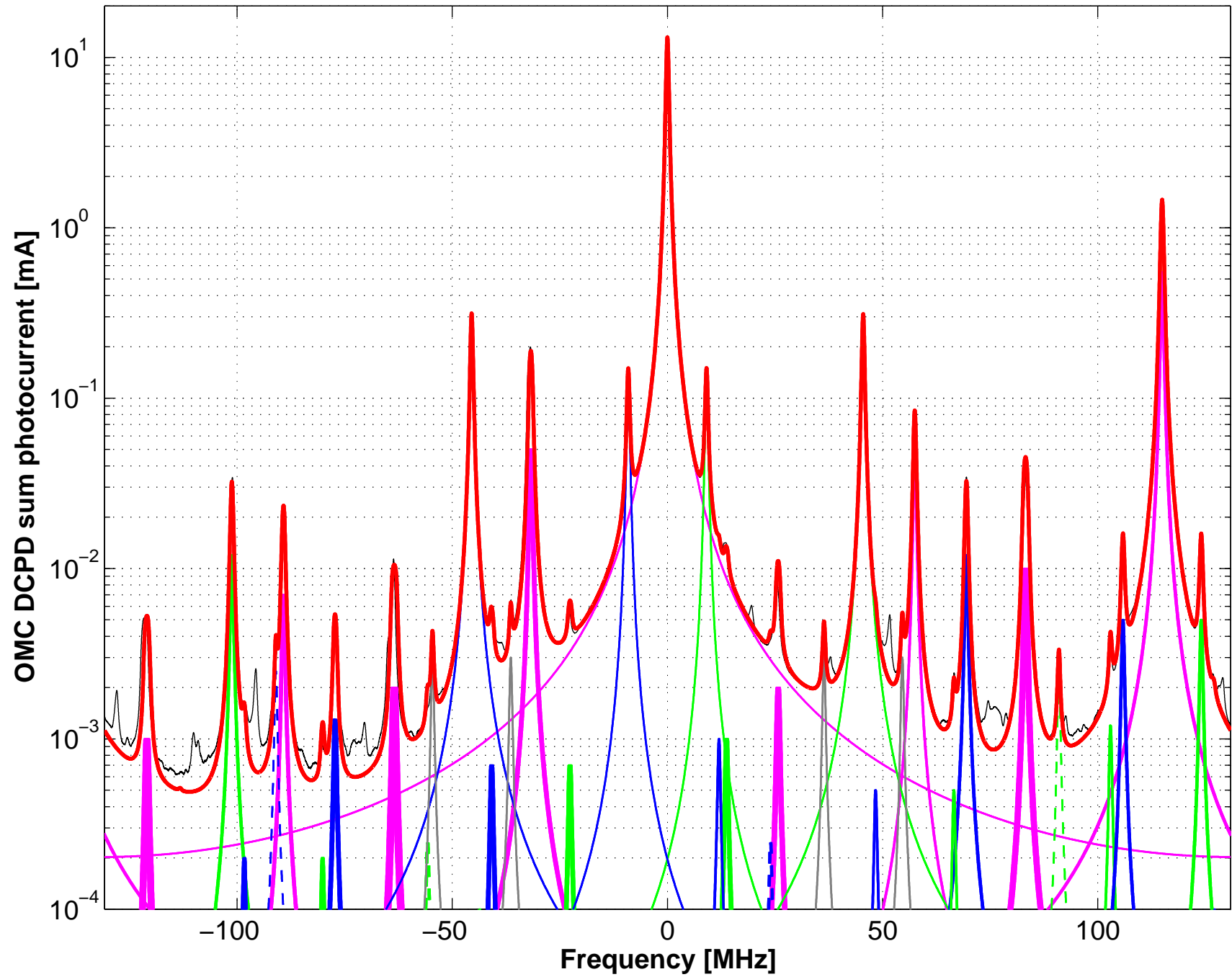
H1 OMC mode scan (ALOG:13660) ~ Peak fitting
