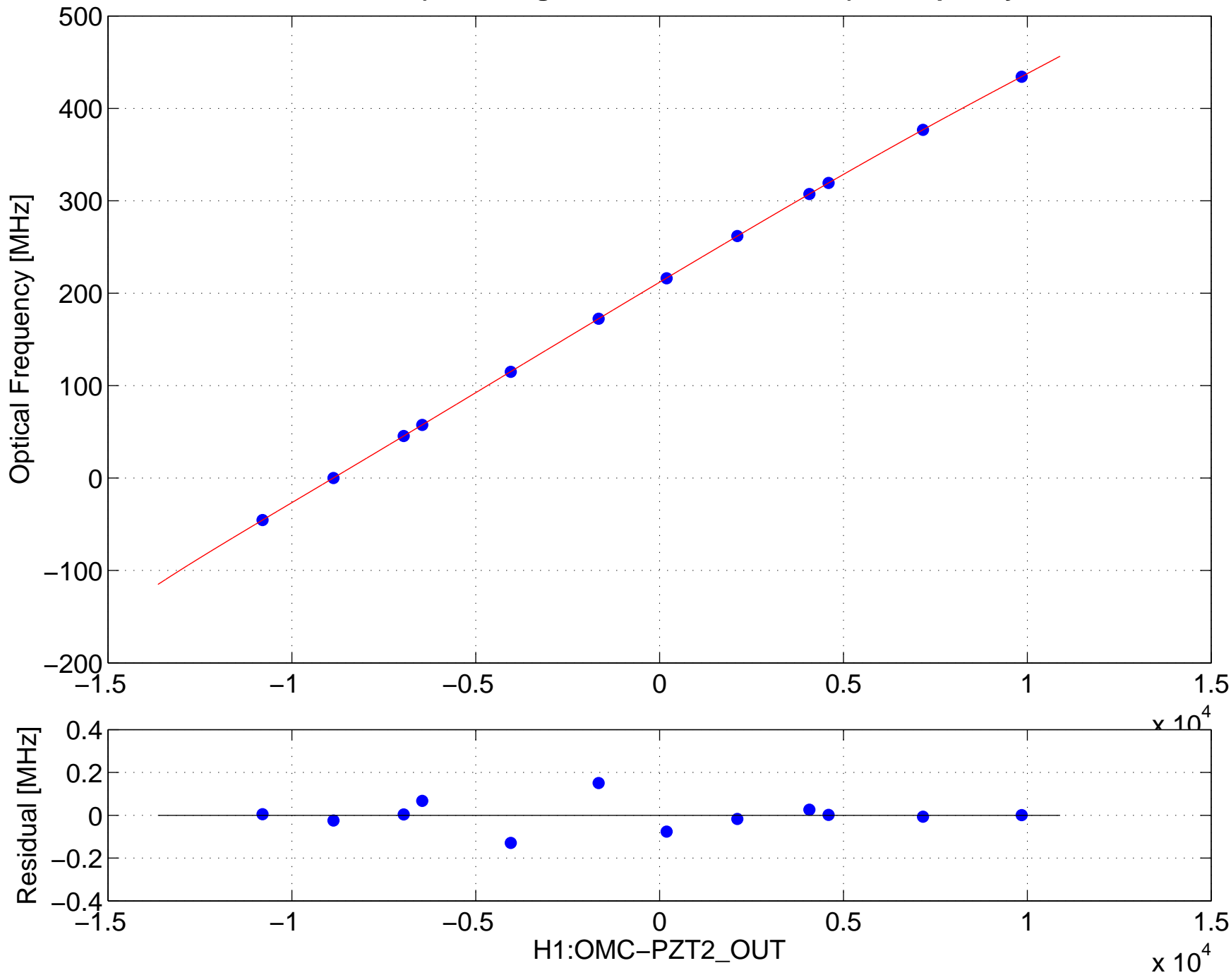
H1 OMC mode scan (ITMY single bounce: ALOG 13799) ~ Frequency Calibration
