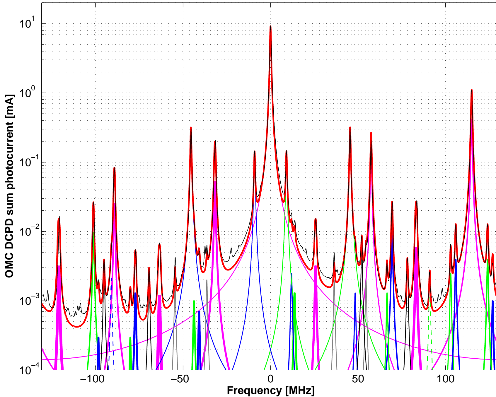
H1 OMC mode scan (ITMY single bounce: ALOG 13799) ~ Peak fitting
