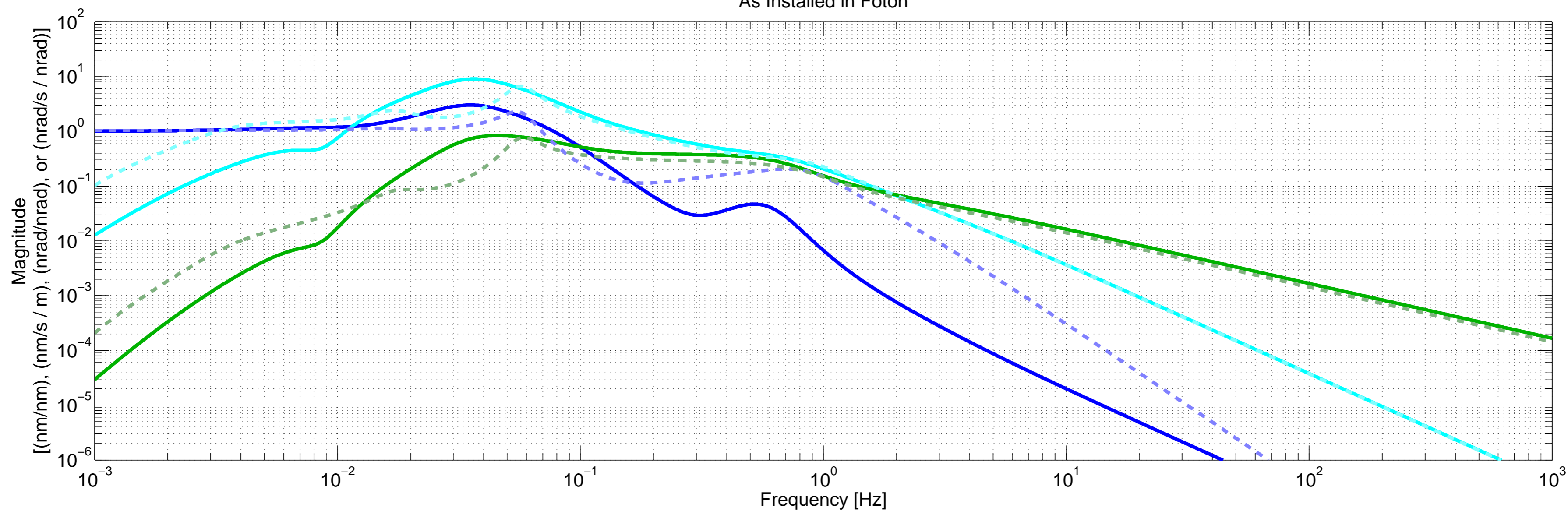
H1ISIITMY ST1 "TBetter" Blend Filters As Installed in Foton
