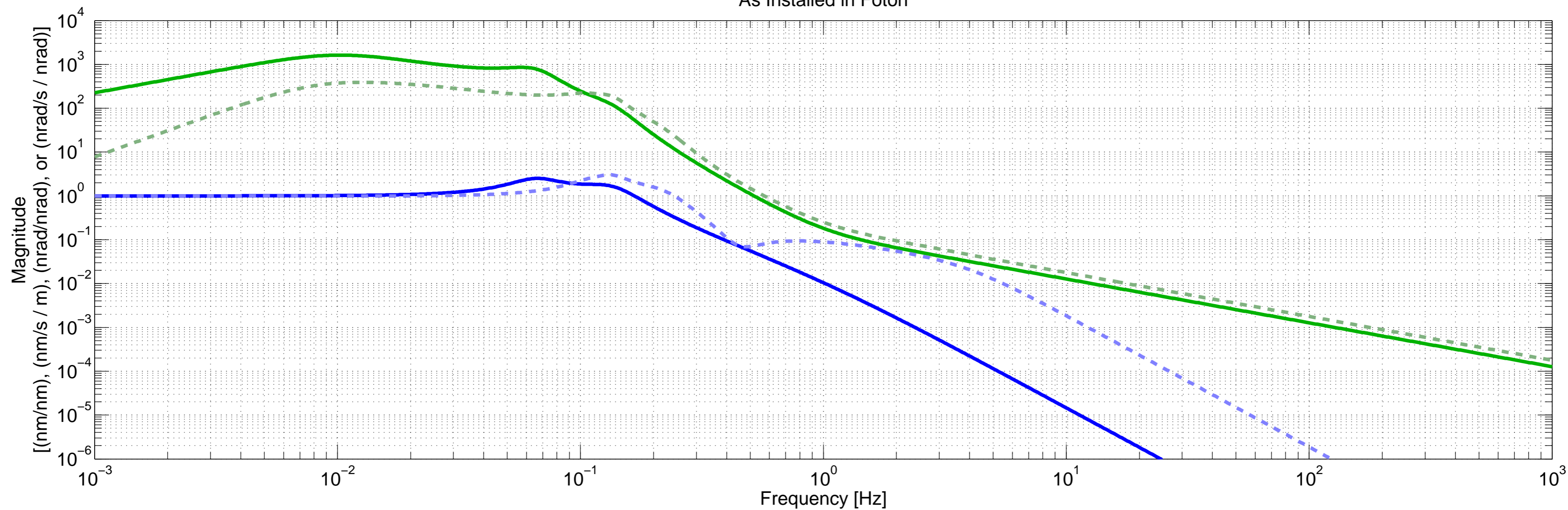
H1ISIITMY ST2 "TBetter" Blend Filters As Installed in Foton
