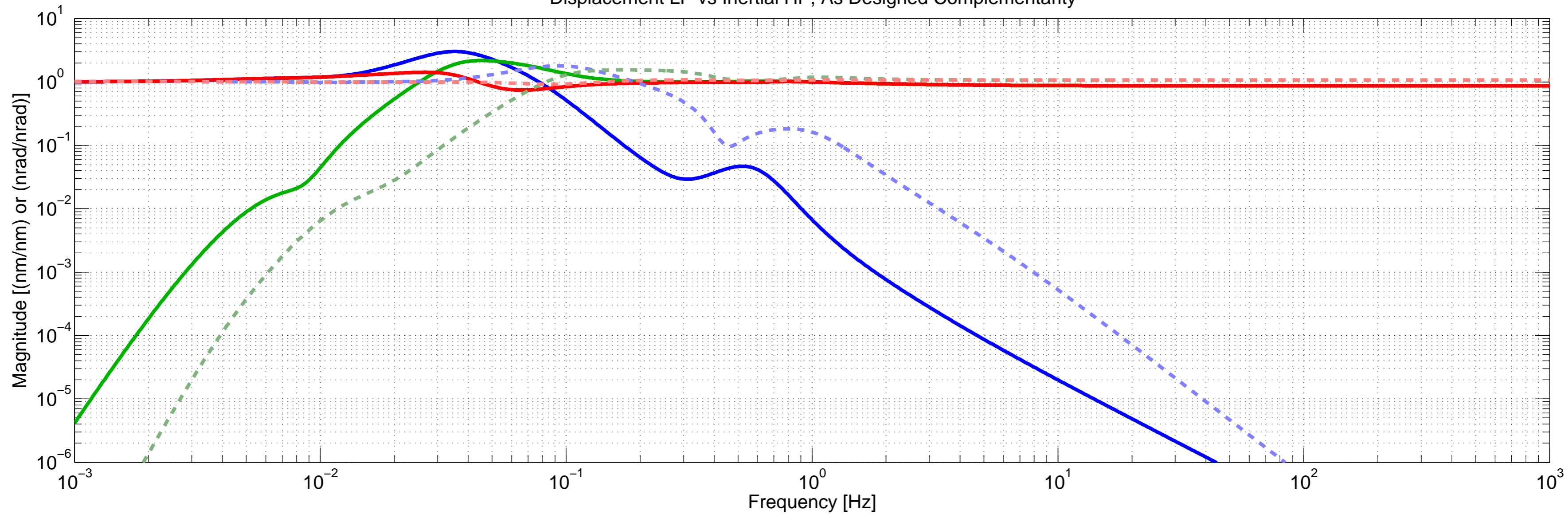
H1ISIITMY ST1 "TBetter" Blend Filters Displacement LP vs Inertial HP, As Designed Complementarity
