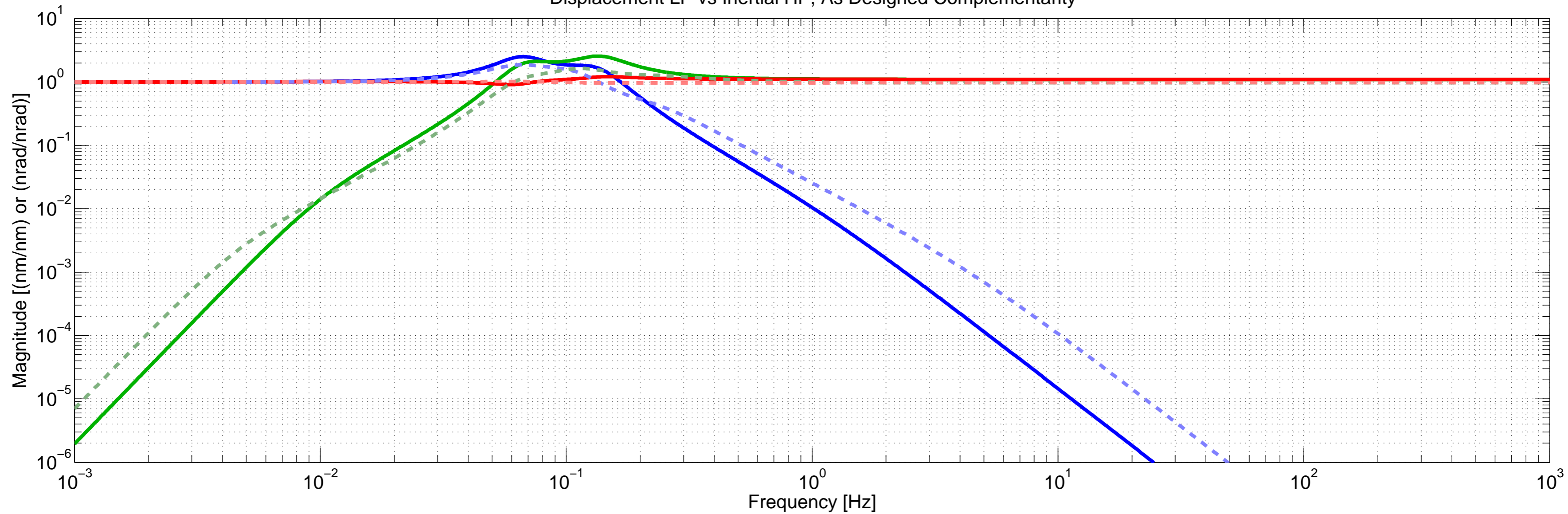
H1ISIITMY ST2 "TBetter" Blend Filters Displacement LP vs Inertial HP, As Designed Complementarity
