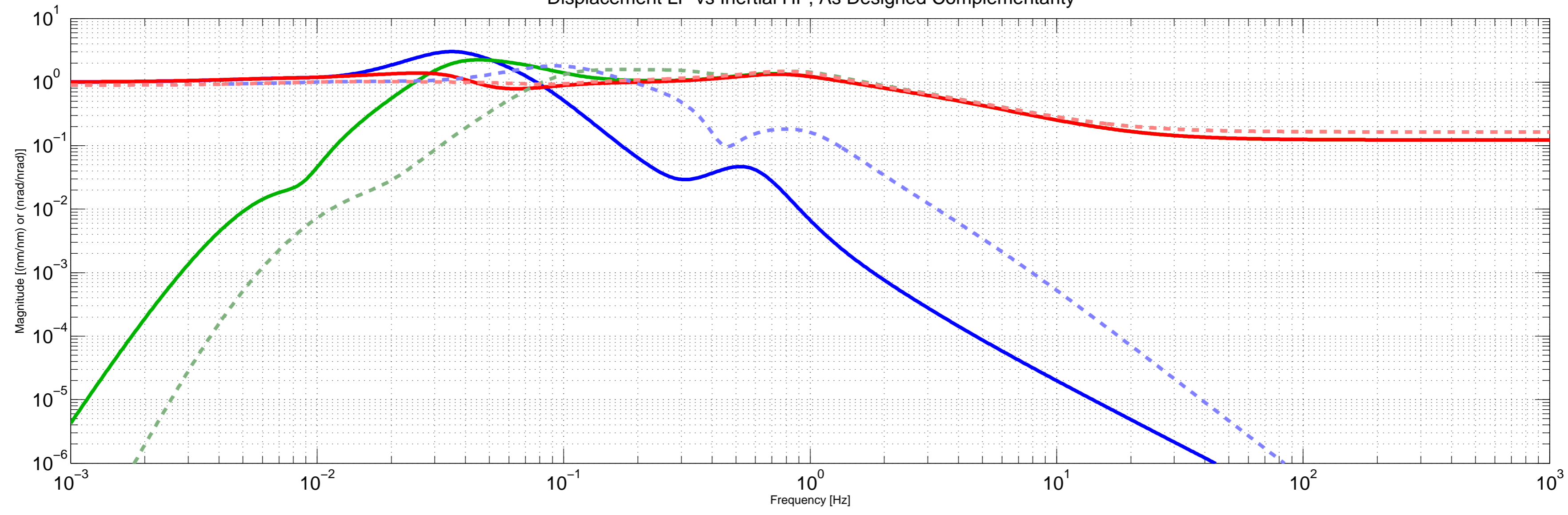
H1ISIITMX ST1 "TSheila" Blend Filters Displacement LP vs Inertial HP, As Designed Complementarity
