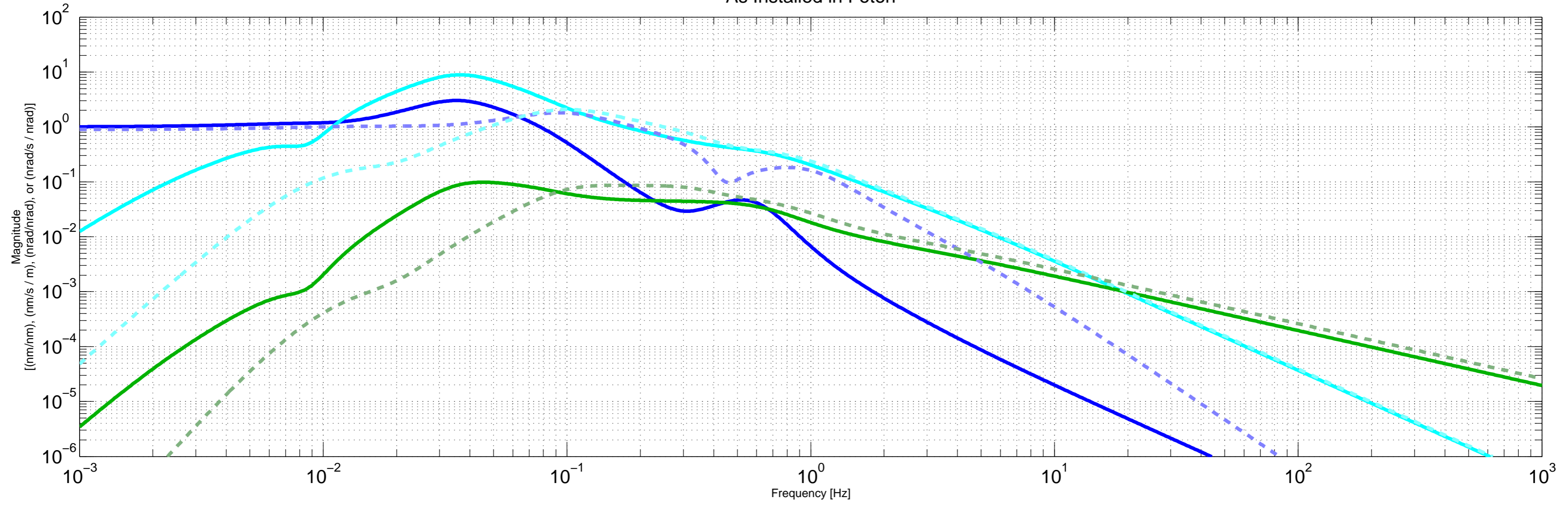
H1ISIITMX ST1 "TSheila" Blend Filters As Installed in Foton
