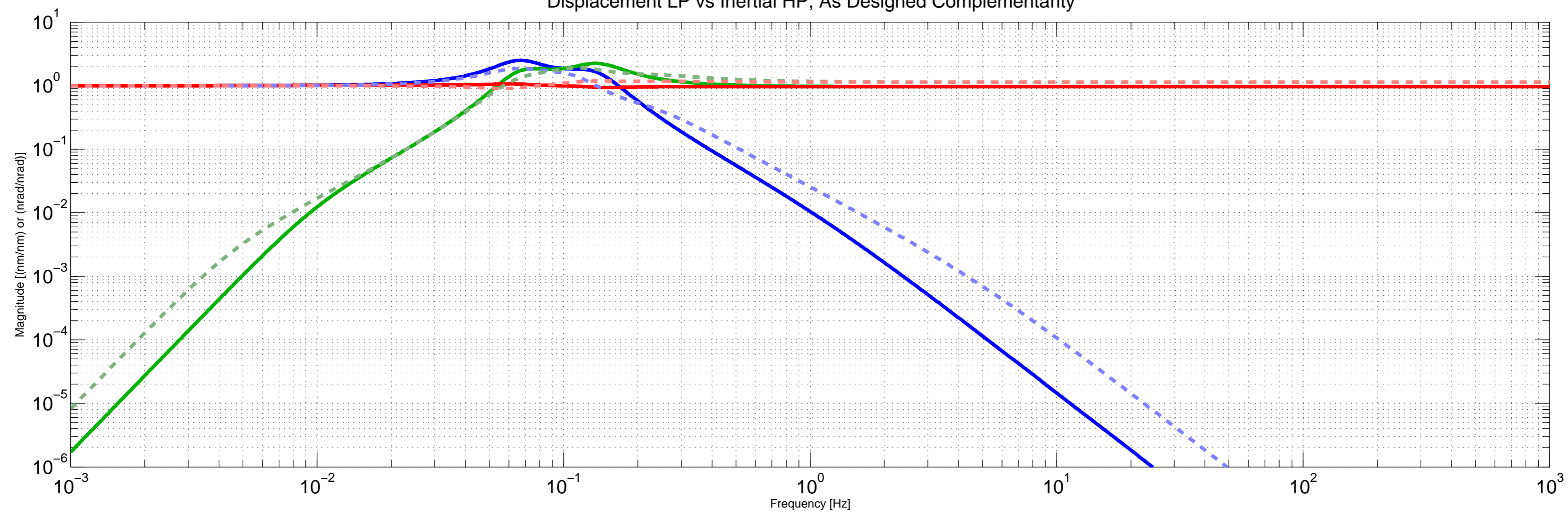
H1ISIITMX ST2 "TSheila" Blend Filters Displacement LP vs Inertial HP, As Designed Complementarity
