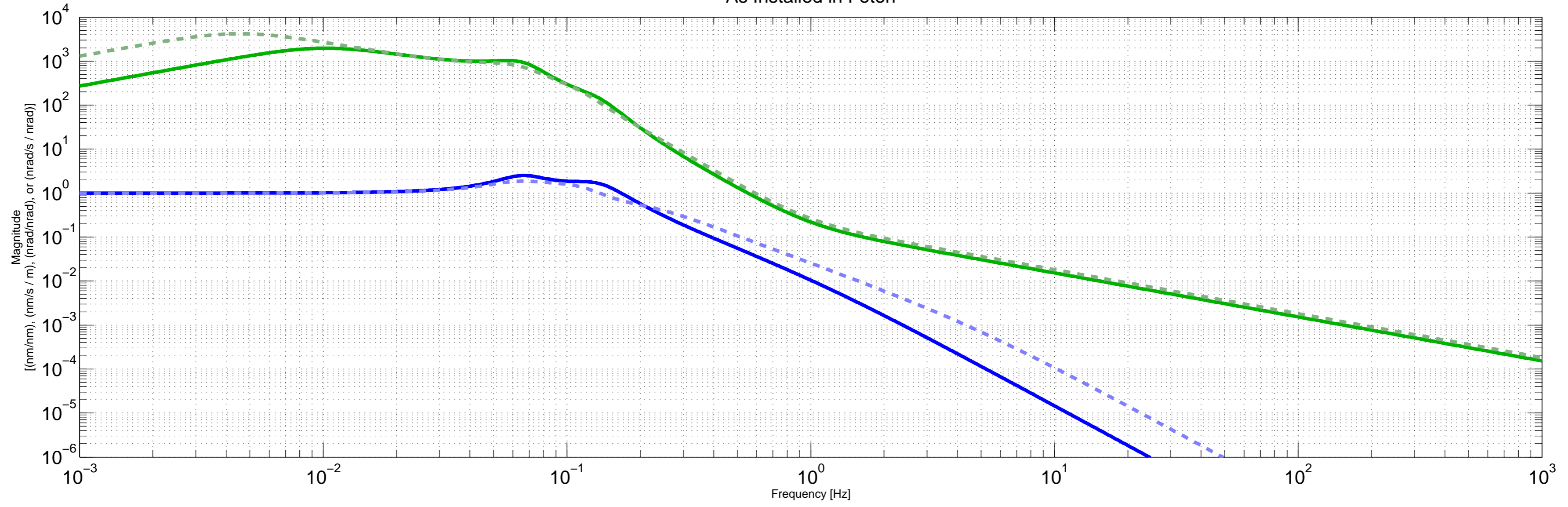
H1ISIITMX ST2 "TSheila" Blend Filters As Installed in Foton
