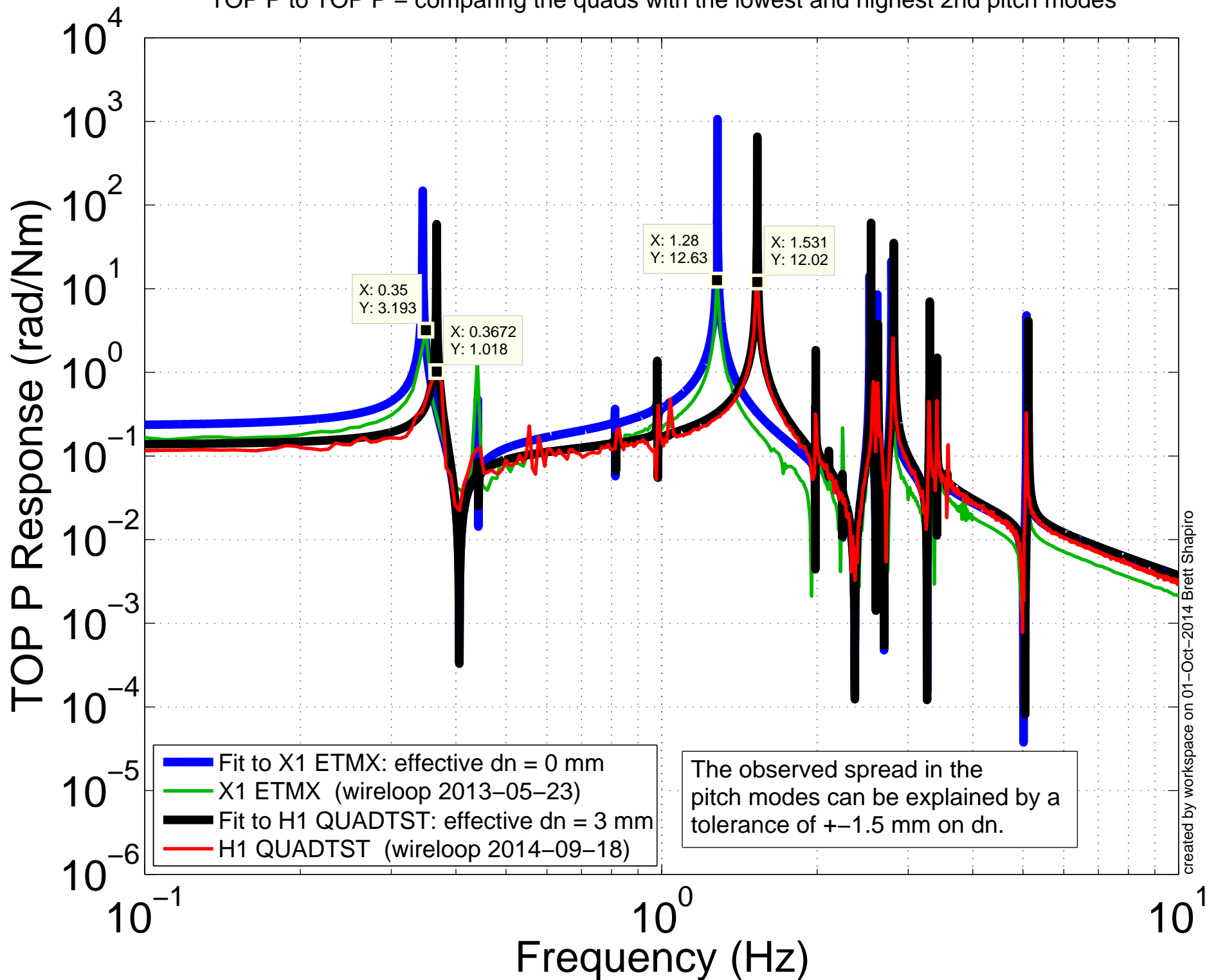
TOP P to TOP P – comparing the quads with the lowest and highest 2nd pitch modes
