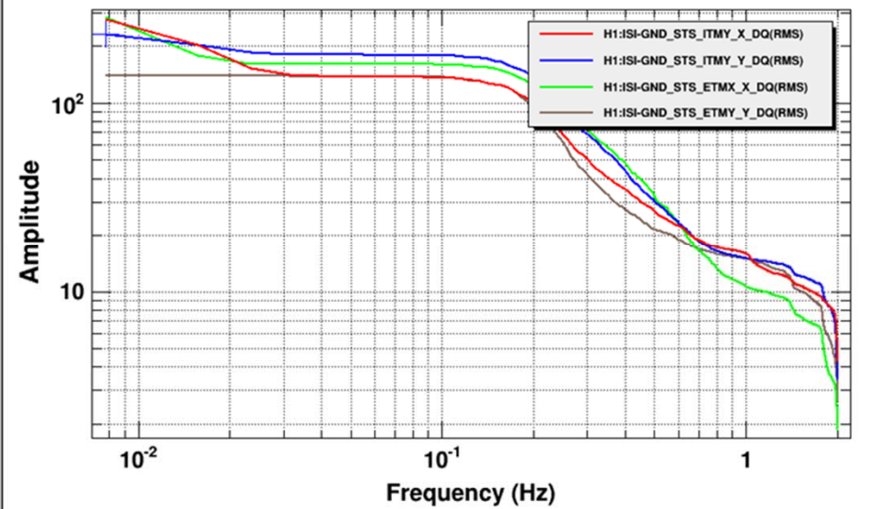
Power spectrum
