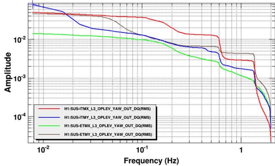
Power spectrum
