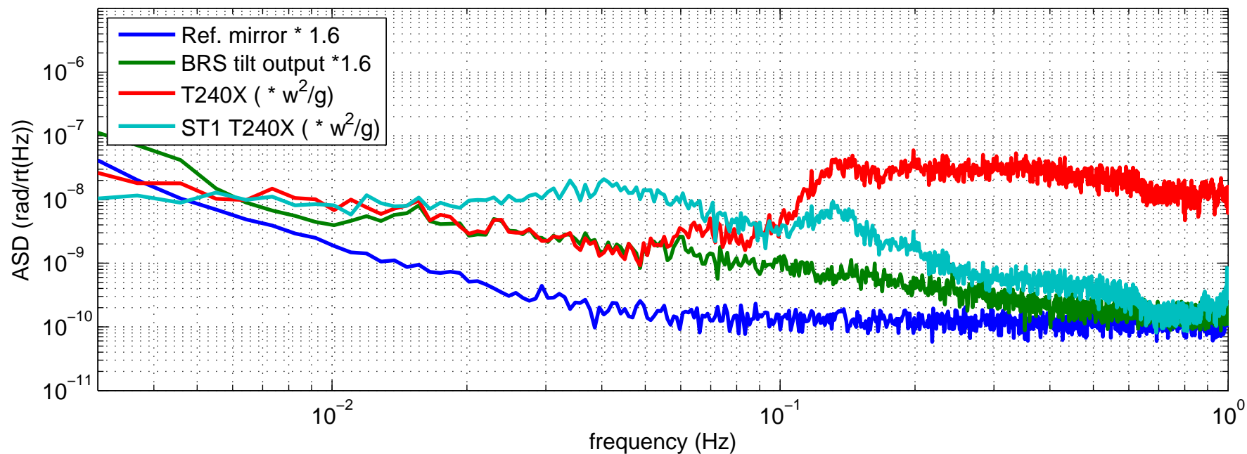
GND T240 and BRS motion compared to ST1 T240X
